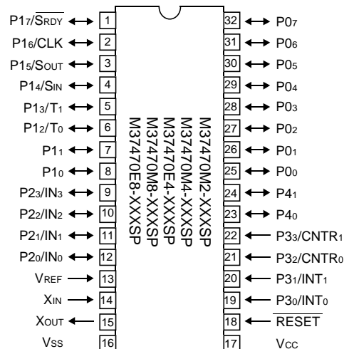
Outline 32P4B
