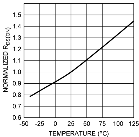
Figure 6-4. Normalized R_{DS(on)} vs Temperature
