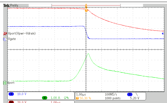
Figure 81. Ports Fast Shutdown from 3-Bit OSS Input
