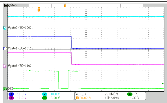
Figure 79. All Ports Power-On With TPON Bit Set
