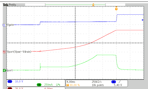
Figure 78. Powering Up into a 100-μF Load
