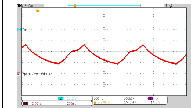
Figure 74. Detection With Invalid PD (15 k \Omega and 0.1 \mu F)
