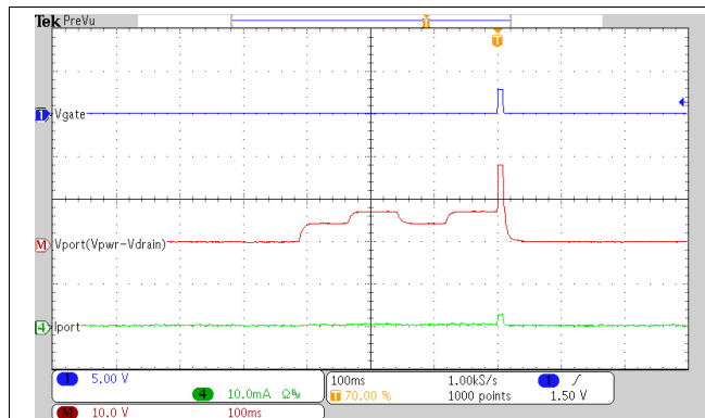
Figure 72. Startup With Valid PD (25 k \Omega and 0.1 \mu F), Class 0
