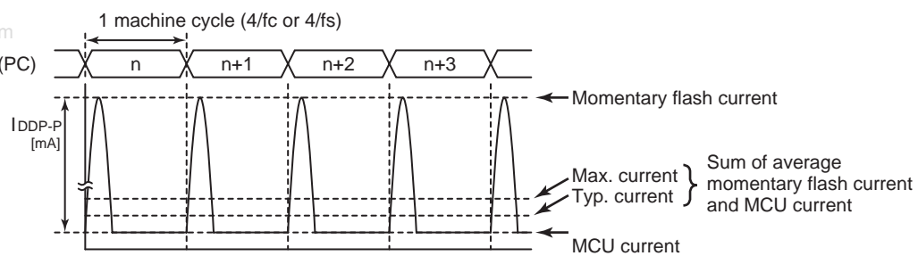
Figure 17-1 Intermittent Operation of Flash Memory
