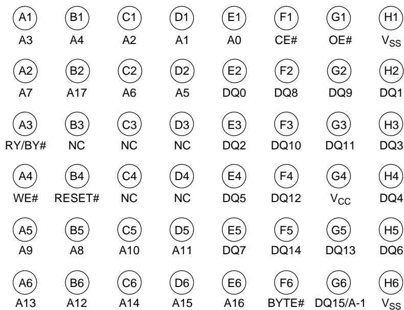
FBGA Bump Side (Bottom) View
