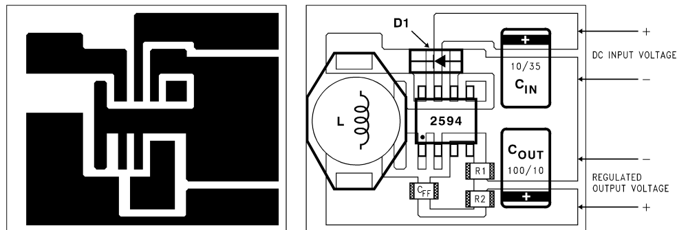
Figure 42. TYPICAL SURFACE MOUNT PC BOARD LAYOUT, ADJUSTABLE OUTPUT (2X SIZE)
