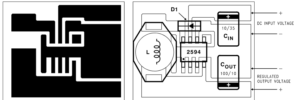
Figure 41. TYPICAL SURFACE MOUNT PC BOARD LAYOUT, FIXED OUTPUT (2X SIZE)
