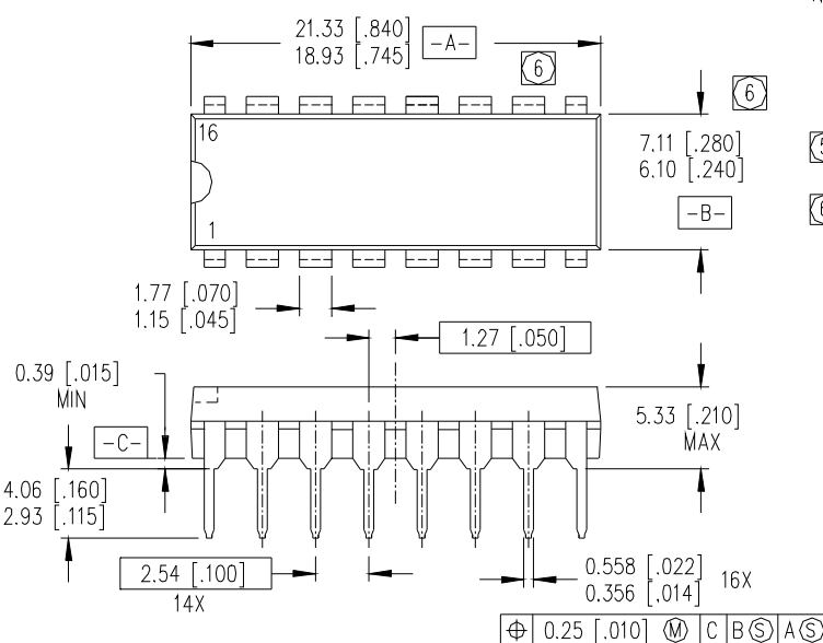
16-Lead PDIP
