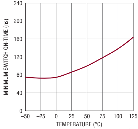
Minimum Switch On-Time vs Temperature
