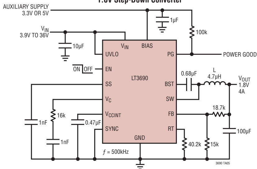
1.8V Step-Down Converter
