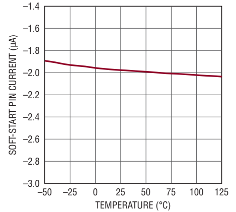
Soft-Start Pin Current
