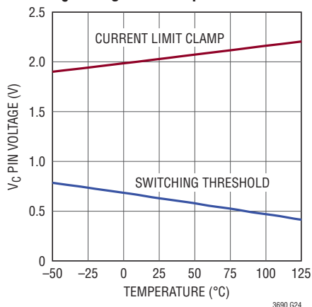
V_C Voltages vs Temperature
