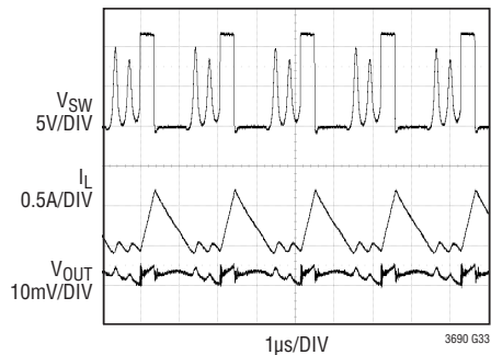
Switching Waveforms, Transition from Burst Mode Operation to Full Frequency
