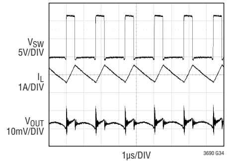
Switching Waveforms, Full Frequency Continuous Operation
