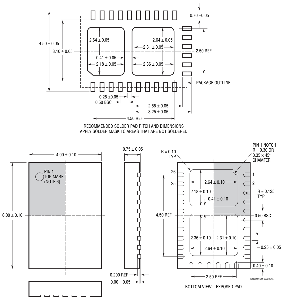
UFE Package 26-Lead Plastic QFN (4mm × 6mm) (Reference LTC DWG # 05-08-1770 Rev A)
