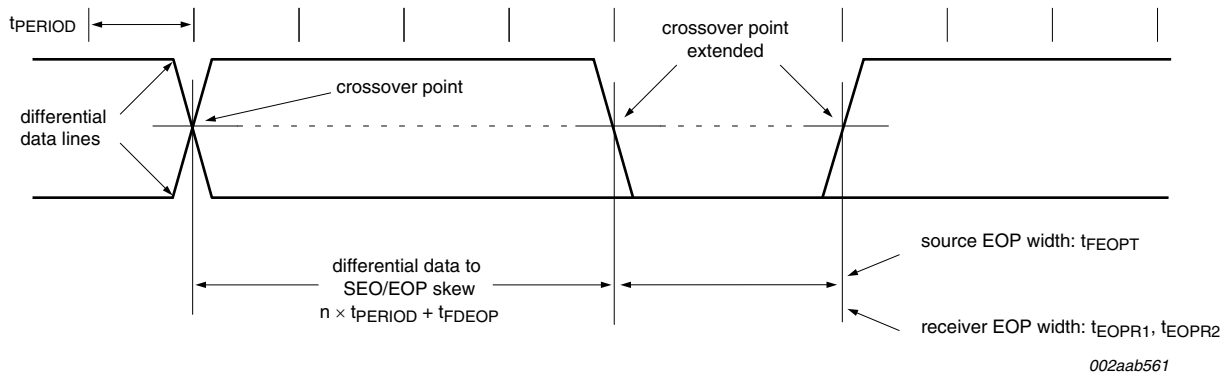
Fig 10. Differential data-to-EOP transition skew and EOP width
