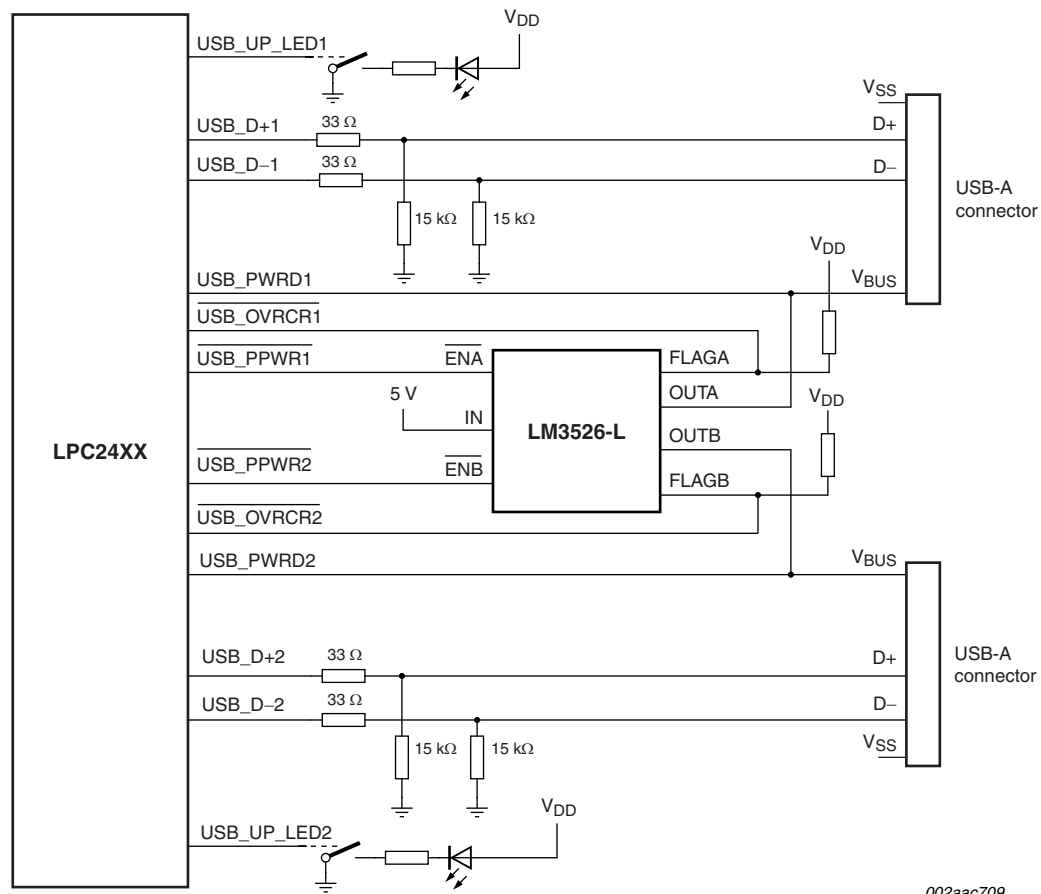
Fig 16. LPC2478 USB OTG port configuration: USB port 1 host, USB port 2 host
