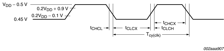
Fig 9. External clock timing
