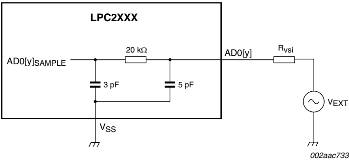
Fig 6. Suggested ADC interface - LPC2478 AD0[y] pin
