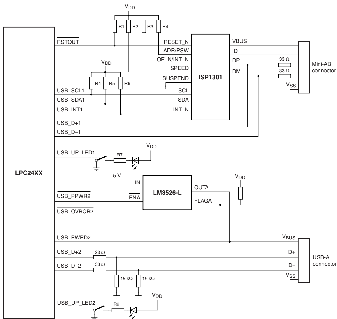
Fig 13. LPC2478 USB OTG port configuration: USB port 1 OTG dual-role device, USB port 2 host
