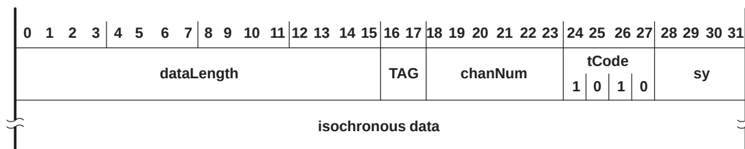
Figure 7–8. Isochronous-Transmit Format
