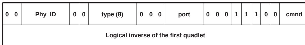
Figure 7–15. Remote Command Packet Format
