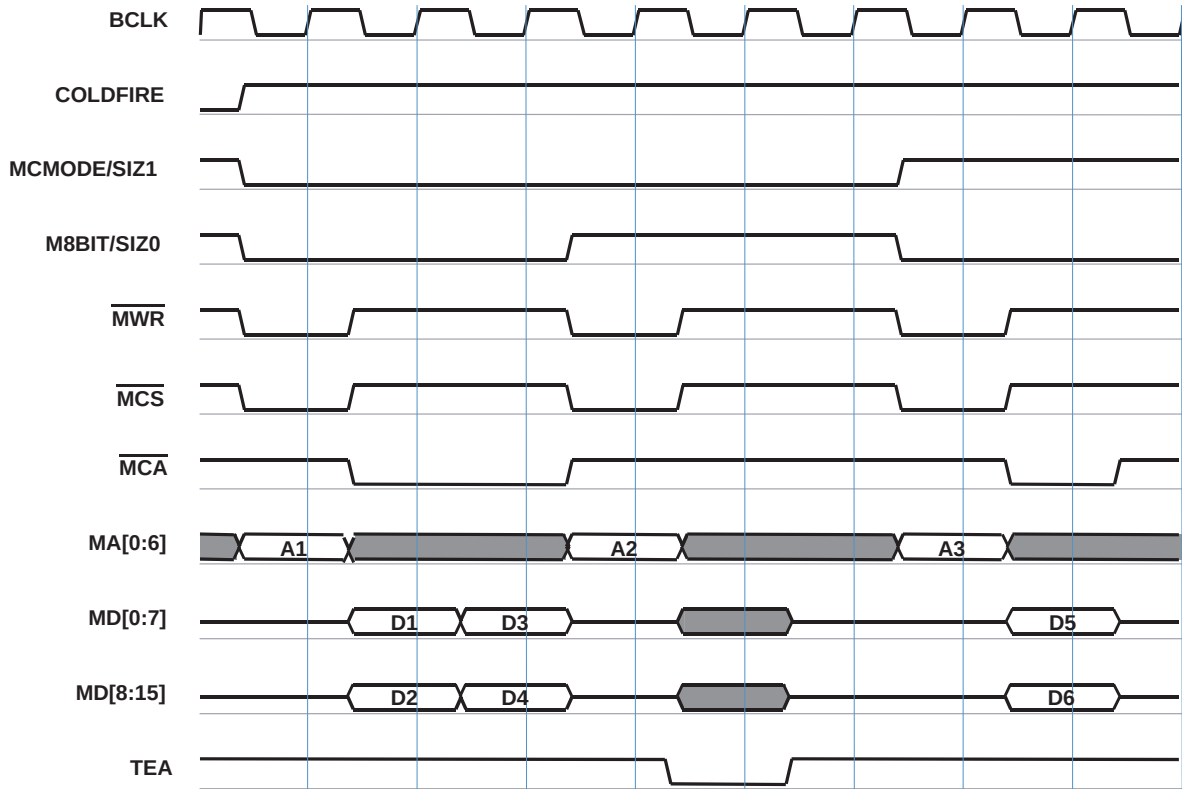
Figure 3–14. ColdFire Write
