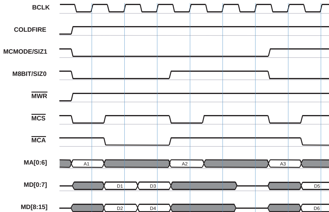
Figure 3–13. ColdFire Read
