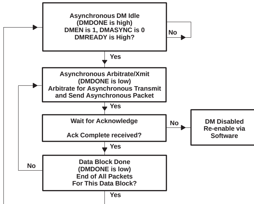
Figure 5-4. Asynchronous DM Flow Control (TSB12LV32 Transmit)
