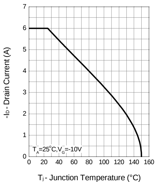
Drain Current
