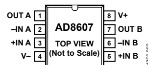
Figure 3. 8-Lead SOIC (R Suffix)
