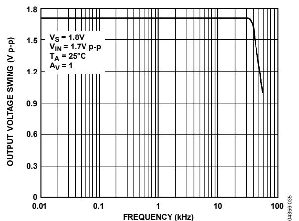
Figure 35. Closed-Loop Output Voltage Swing vs. Frequency
