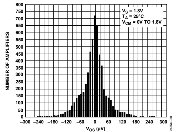
Figure 28. V_{OS} Distribution
