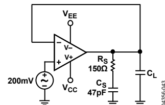
Figure 43. Snubber Network
