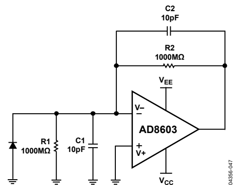
Figure 47. Photodiode Circuit
