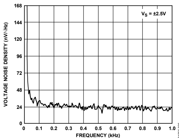
Figure 26. Voltage Noise Density vs. Frequency
