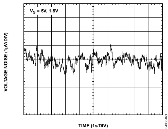
Figure 21. 0.1 Hz to 10 Hz Input Voltage Noise
