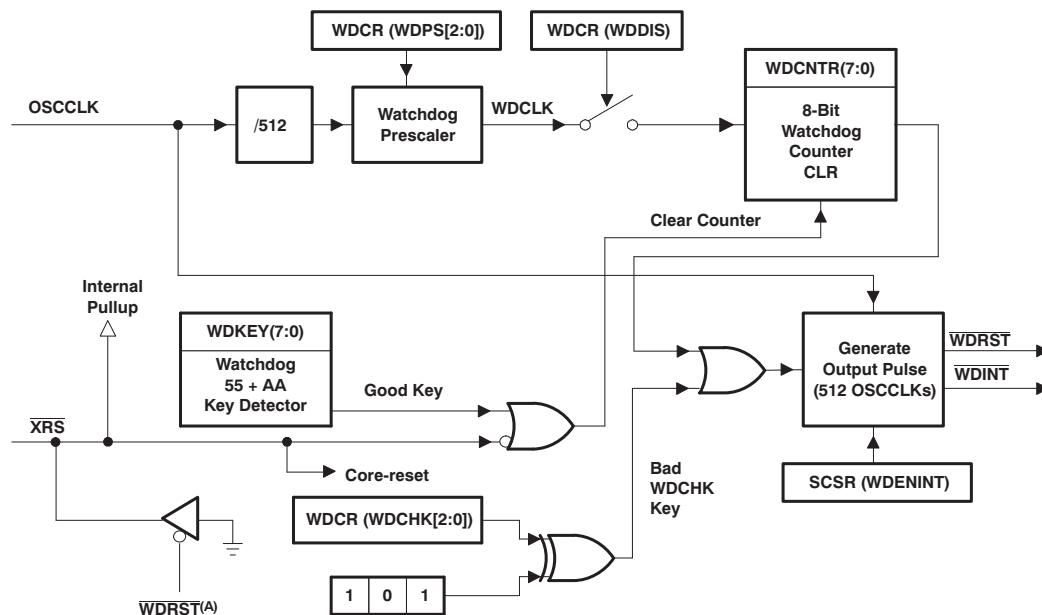
Figure 3-11. Watchdog Module
