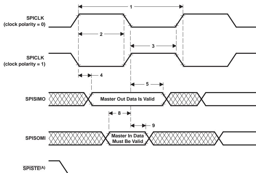
Figure 6-19. SPI Master Mode External Timing (Clock Phase = 0)
