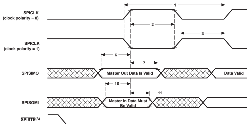
Figure 6-20. SPI Master Mode External Timing (Clock Phase = 1)
