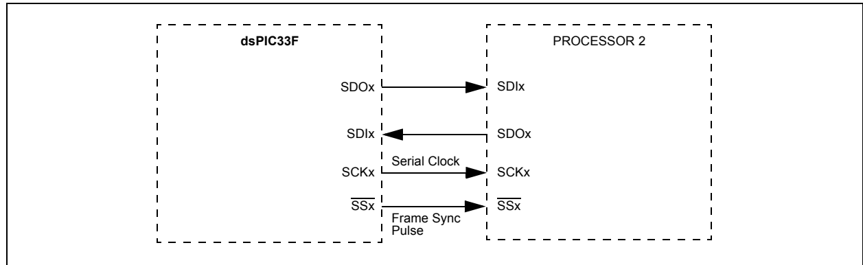
FIGURE 16-3: SPI MASTER, FRAME MASTER CONNECTION DIAGRAM
