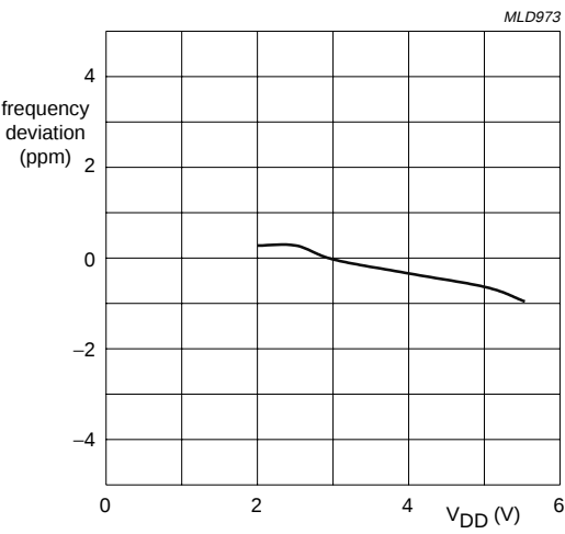
Fig 18. Frequency deviation as a function of V_{DD} .
