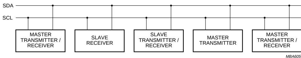
Fig 8. System configuration.
