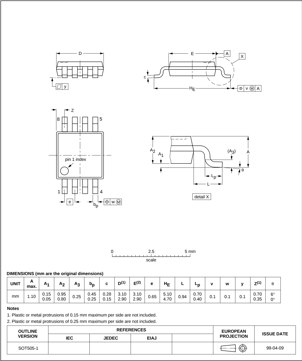
Fig 20. Package outline.
