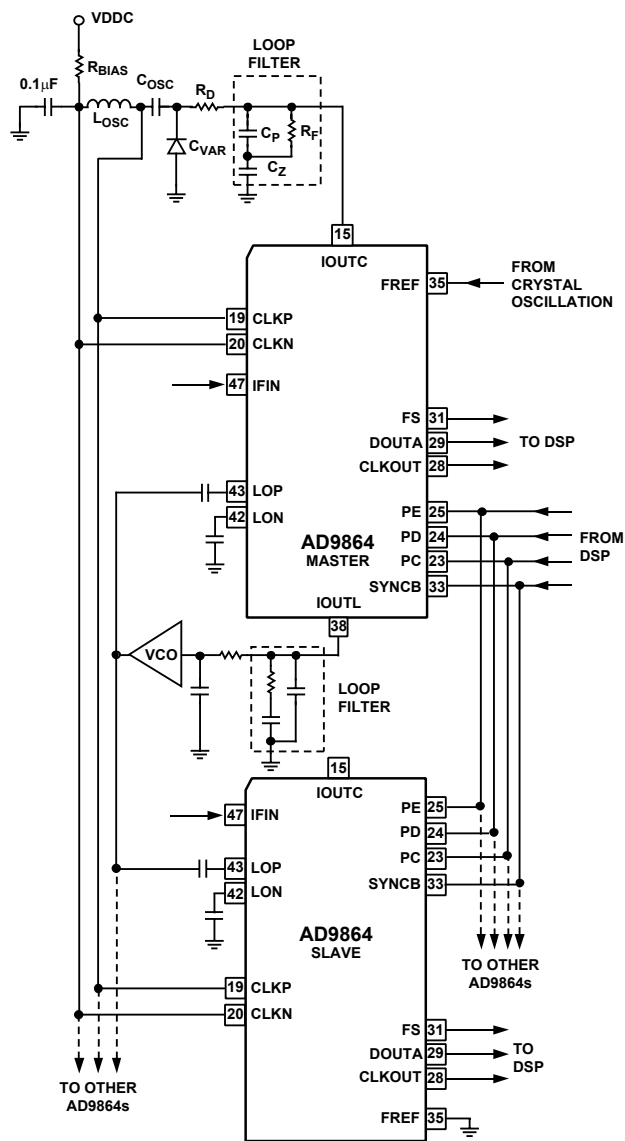
Figure 72. Example of Synchronizing Multiple AD9864s
