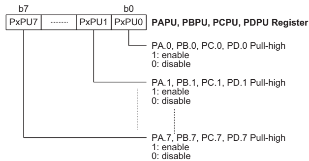
Pull-High Resistor Register – PAPU, PBP, PCPU, PDP
