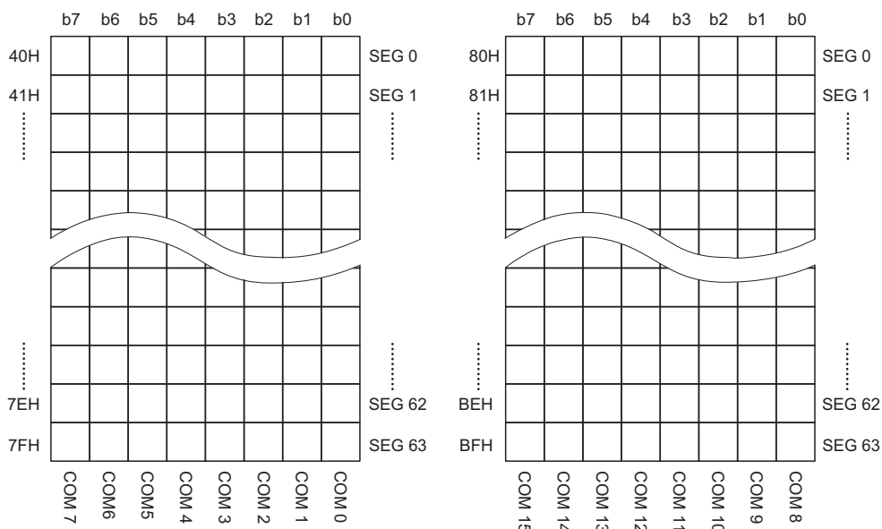
HT56R678 Memory Map – 64×16
