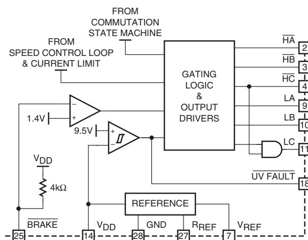
Figure 10. Cross Conduction, Brake, and UVLO Circuits
