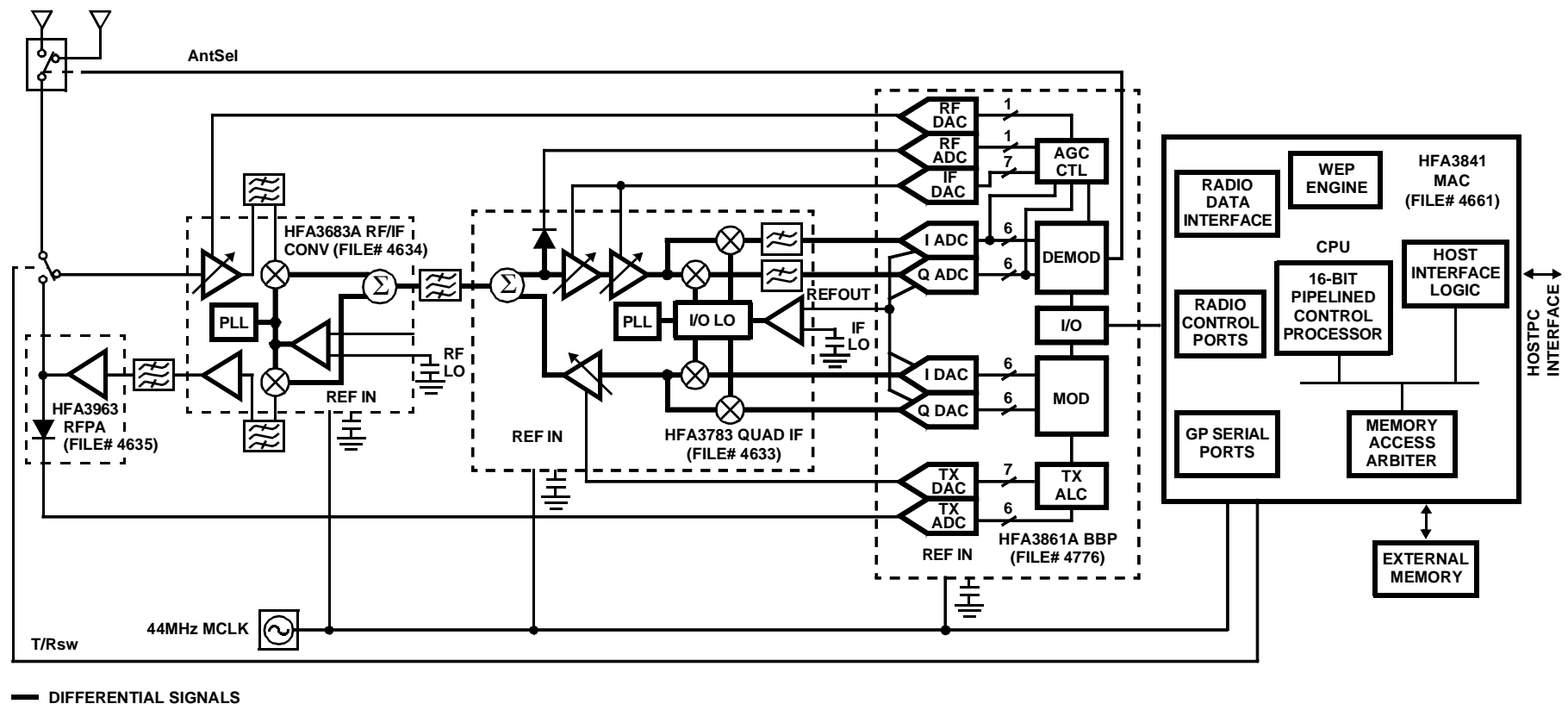
TYPICAL TRANSCEIVER APPLICATION CIRCUIT USING THE HFA3861A
