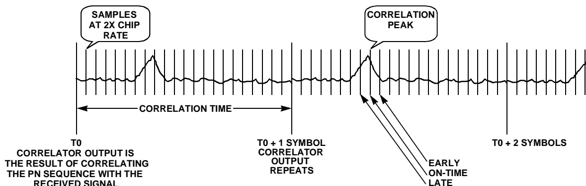
FIGURE 12. CORRELATION PROCESS
