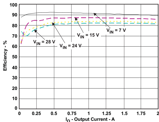
Figure 15. TPS54231 Efficiency
