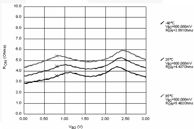
Figure 8. R_{ON}
