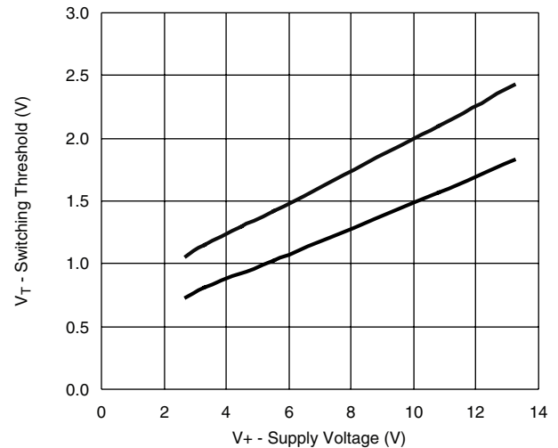
Switching Threshold vs. Supply Voltage
