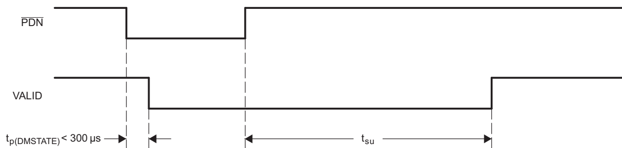
Figure 7-5. Power-Down Timing
