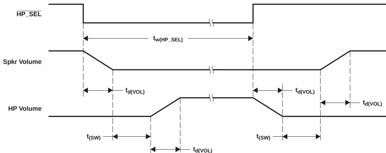
Figure 7-8. \overline{\text{HP\_SEL}} Timing
