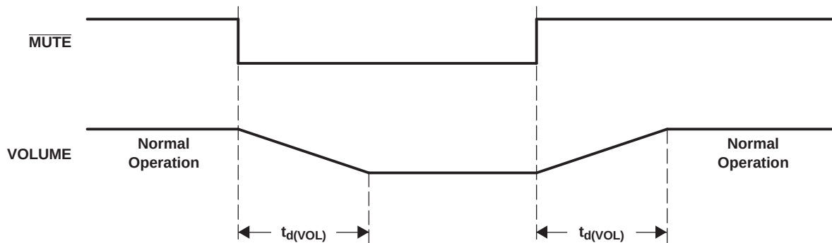
Figure 7-7. Mute Timing
