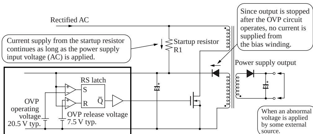
Figure 10. OVP operating circuit
