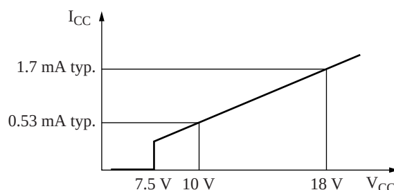
Figure 11. OVP operating circuit current
