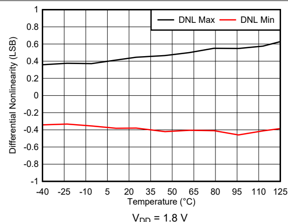
Figure 5-10. Differential Nonlinearity vs Temperature
