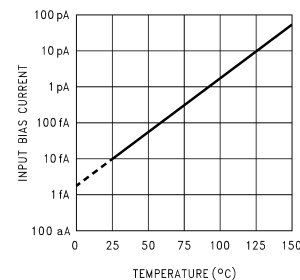
Figure 2. Input Bias Current vs Temperature
