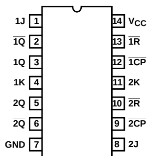
CD74HC107, CD74HCT107 (PDIP, SOIC) TOP VIEW
