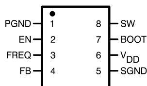
Figure 1. VSSOP-8 (DGK) Package - Top View
