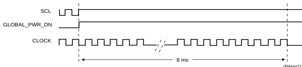
Fig 6. Clock stopped using the GLOBAL_PWR_DN bit.
