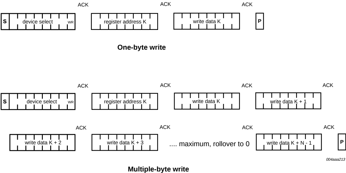
Fig 12. Writing data to the ISP1301 registers.
