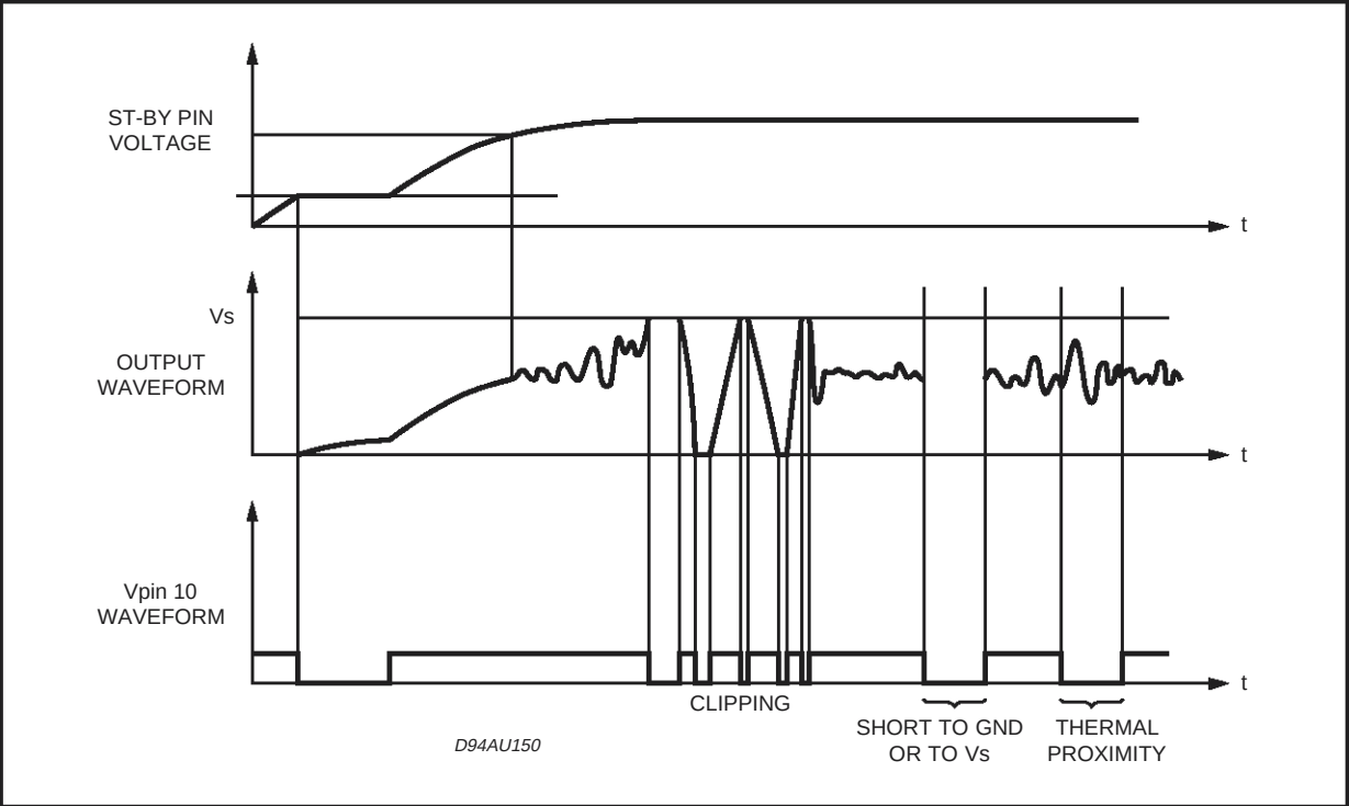
Figure 25: Waveforms
