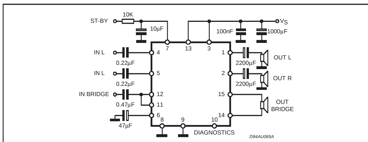
Figure 3: Stereo/Bridge
