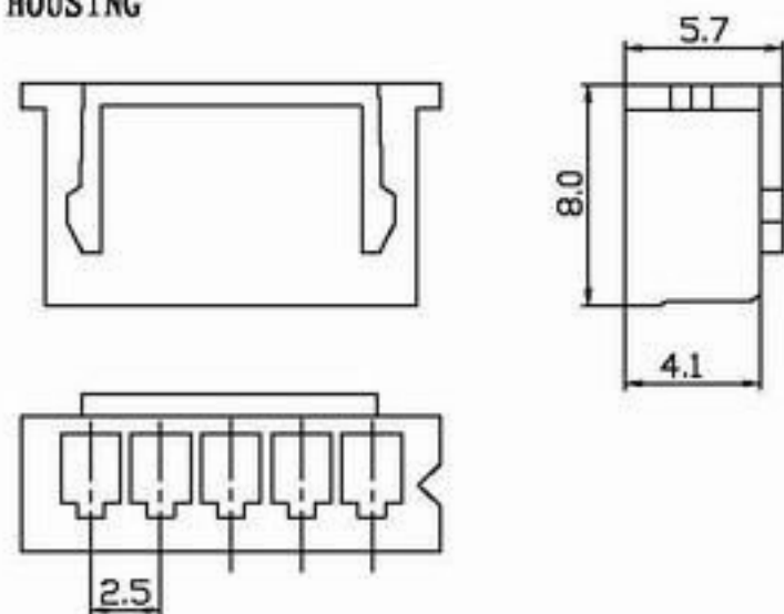
阴连接器 HOUSING
