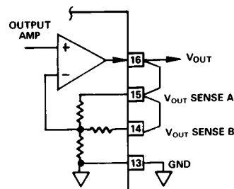
Figure 2. 0 V to 2.56 V Output Range
