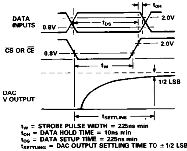
Figure 7. AD557 Timing
