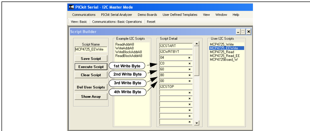
FIGURE 9-3: Example of PICKit™ Serial User Interface.
