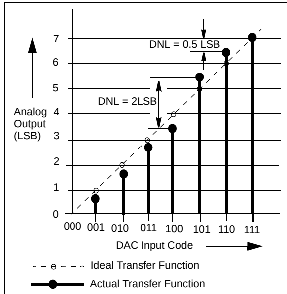
FIGURE 4-2: DNL Accuracy.
