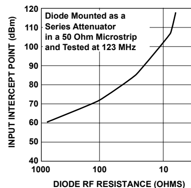
Figure 3. 2nd Harmonic Input Intercept Point vs. Diode RF Resistance.
