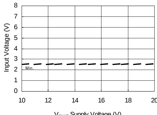
Figure 12B. Logic "1" Input Voltage vs. Voltage
