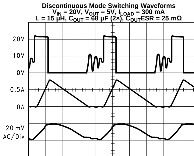
Figure 19. Horizontal Time Base: 1 \mu\text{s/div}
