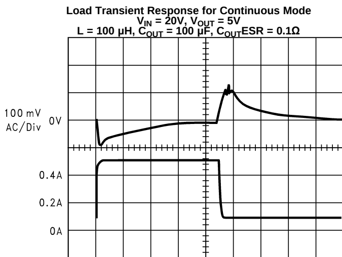
Figure 18. Horizontal Time Base: 1 \mu\text{s/div}
