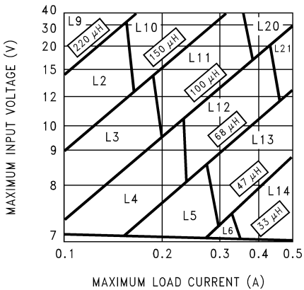
Figure 25. LM2671-5.0
