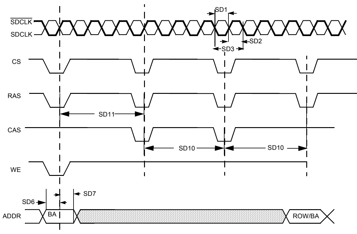
Figure 39. SDRAM Refresh Timing Diagram
