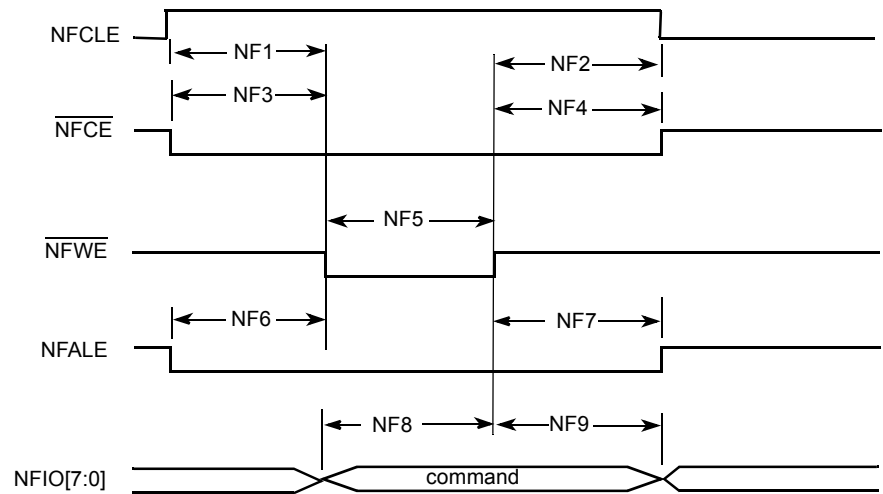
Figure 31. Command Latch Cycle Timing Diagram
