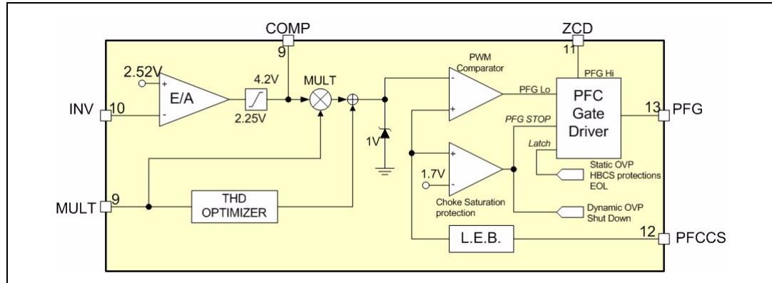
Figure 4. PFC section
