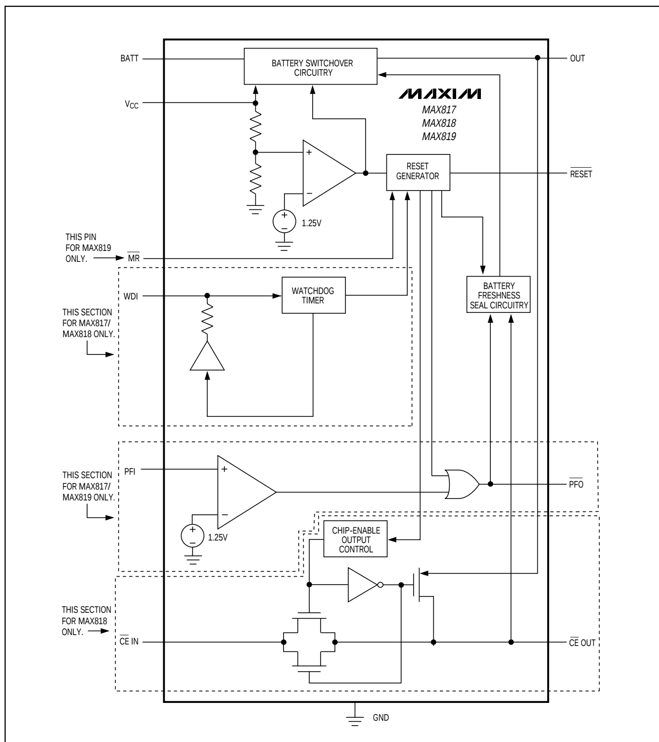
Figure 1. Functional Diagram
