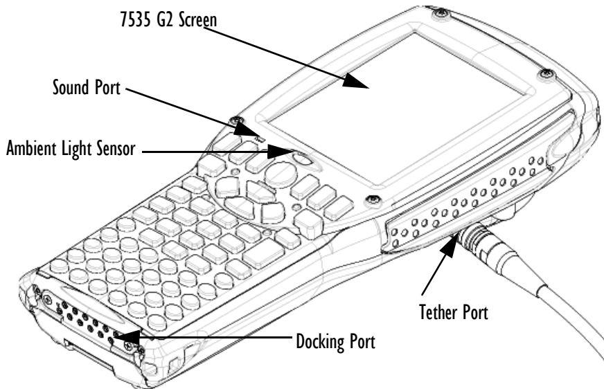
Figure 3.1 Front Of 7535 G2
