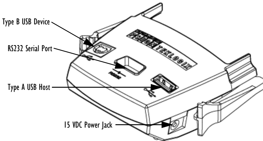
Figure 6.2 PDM Ports And Connectors
