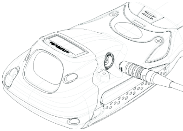
Figure 3.8 Attaching The Cable To The Tether Port
