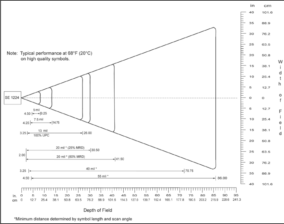
Figure 7.2 SE 1224HP Decode Zones
