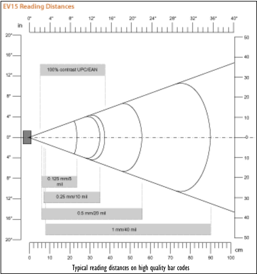
Figure 7.1 EV15 Decode Zones
