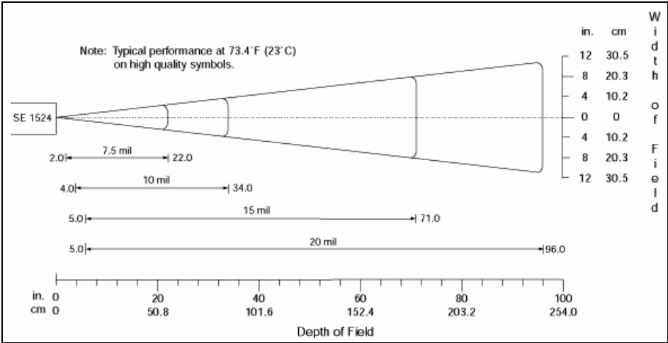
Figure 7.3 SE1524ER Decode Zone A (Short Range, Small Codes)
