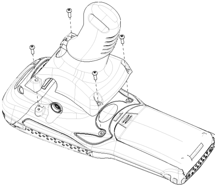
Figure 2.4 Attaching The Pistol Grip
