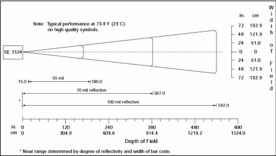
Figure 7.4 SE1524ER Decode Zone B (Long Range, Large Codes)
