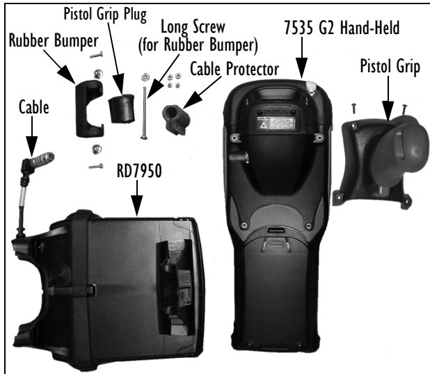
Figure B.1 RD7950 Installation Components
