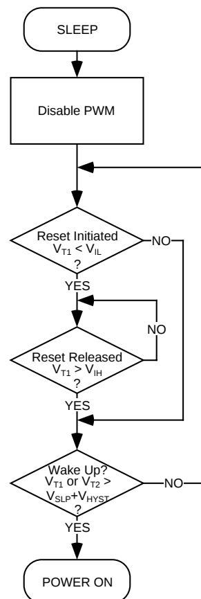
Figure 5. Sleep-Mode Behavior
