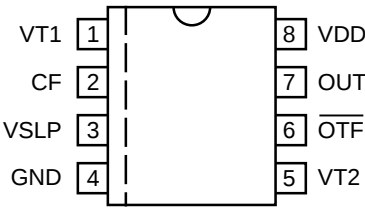
8-Pin SOIC (M) 8-Pin DIP (N)
