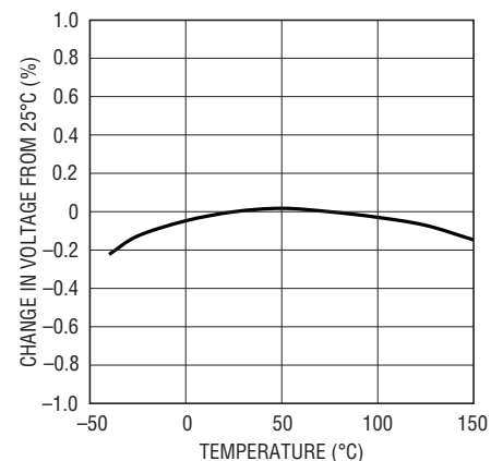
LDO Output Voltage
