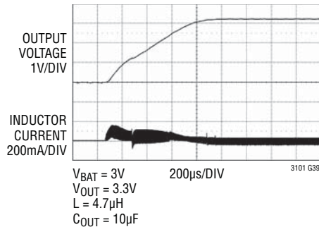
Buck-Boost Soft-Start, PWM Mode
