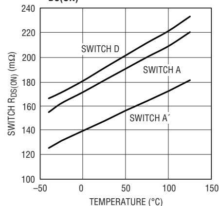
Buck-Boost P-Channel Switch R_{DS(ON)}
