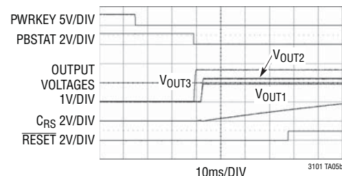
Power-Up Waveforms
