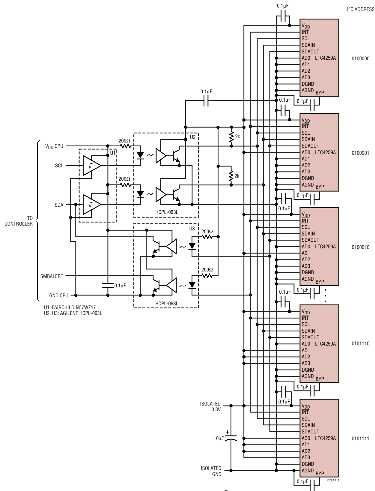
Figure 18. Optoisolating the I 2 C Bus
