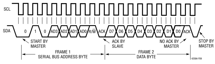
Figure 9. Reading the Interrupt Register (Short Form)
