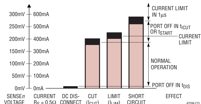
Figure 15. LTC4259A Current Sense and Limits
