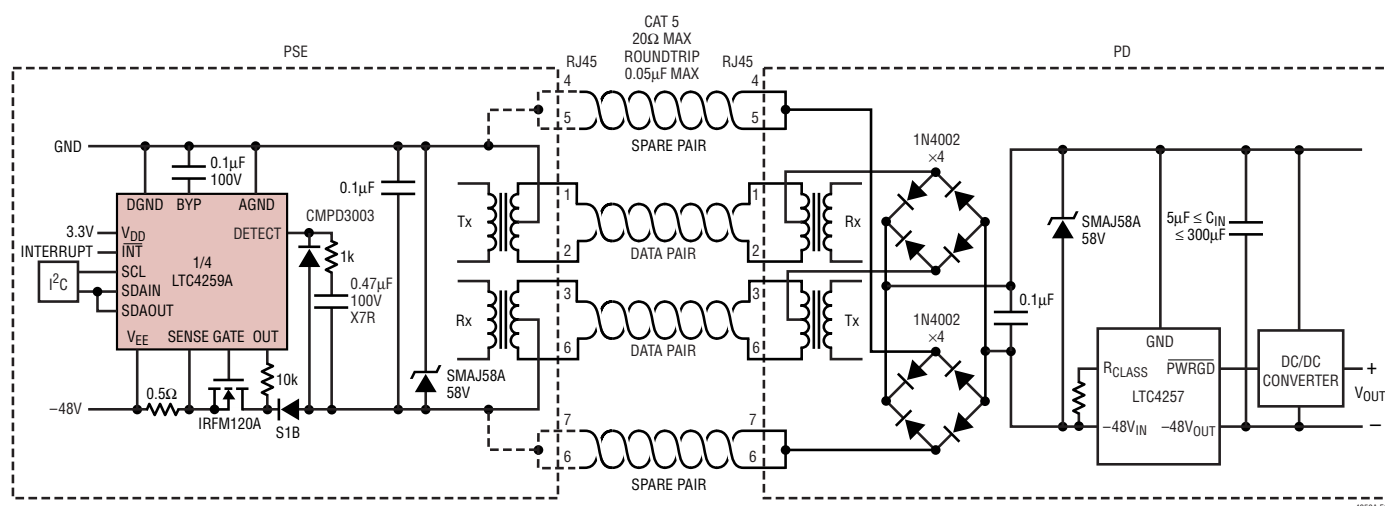
Figure 11. System Diagram
