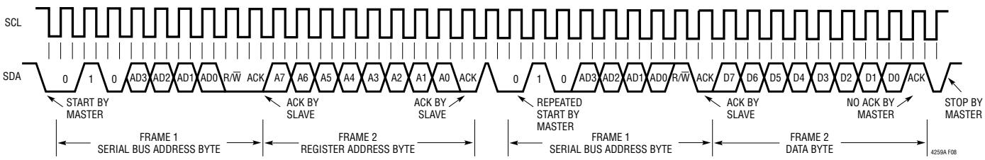
Figure 8. Reading from a Register
