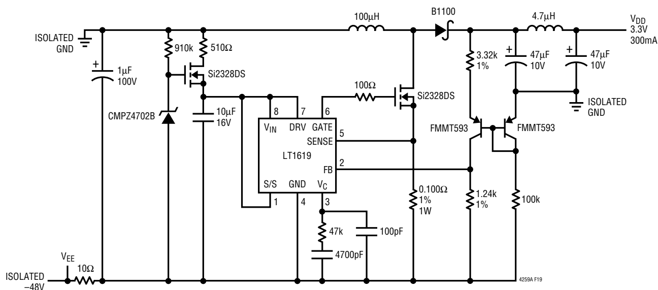
Figure 19. -48\text{V} to 3.3\text{V} Boost Converter
