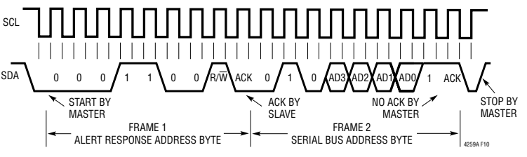
Figure 10. Reading from Alert Response Address
