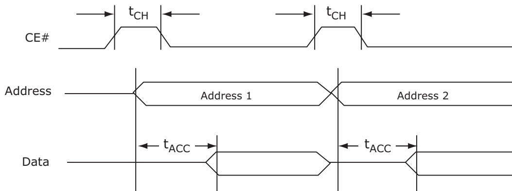
Figure 1. t_{CH} Hold Time
