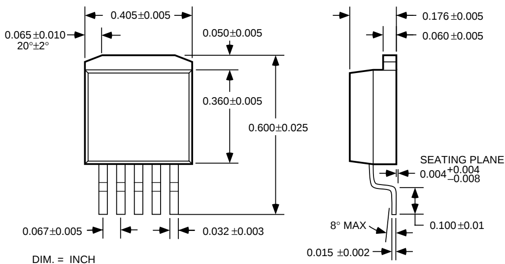
5-Lead TO-263 (U)
