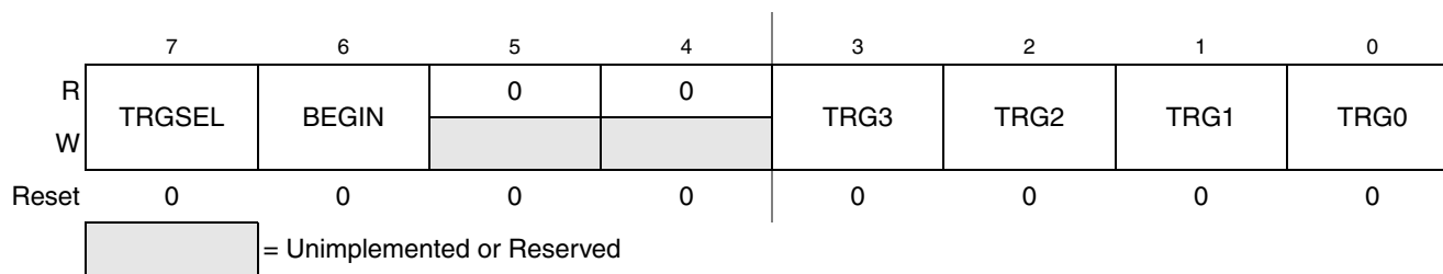
Figure 16-8. Debug Trigger Register (DBGT)
