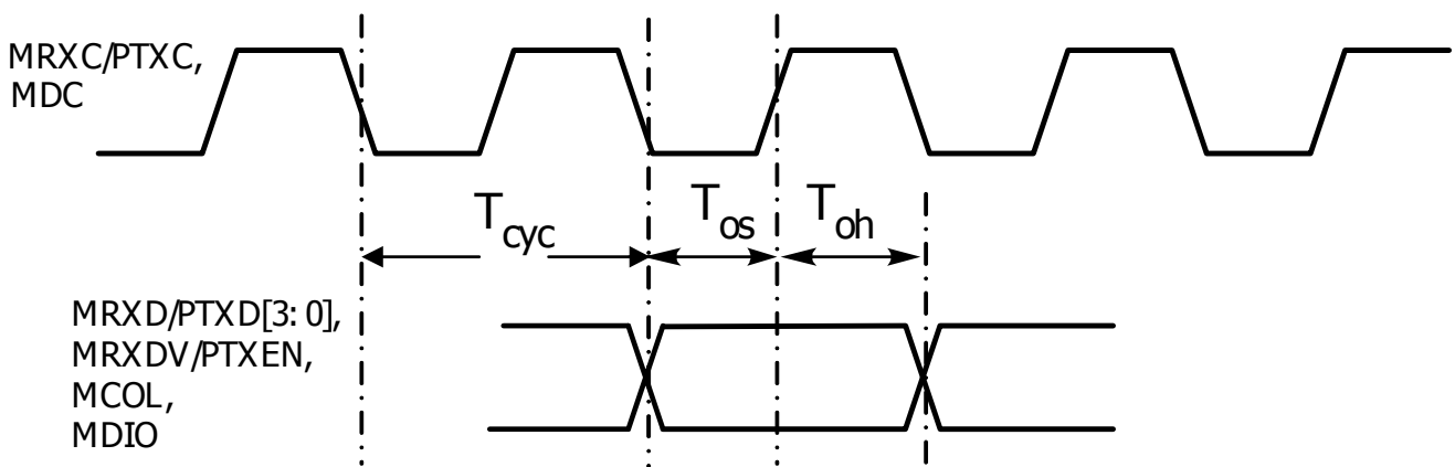
Figure 21. MII Interface Transmission Data Timing
