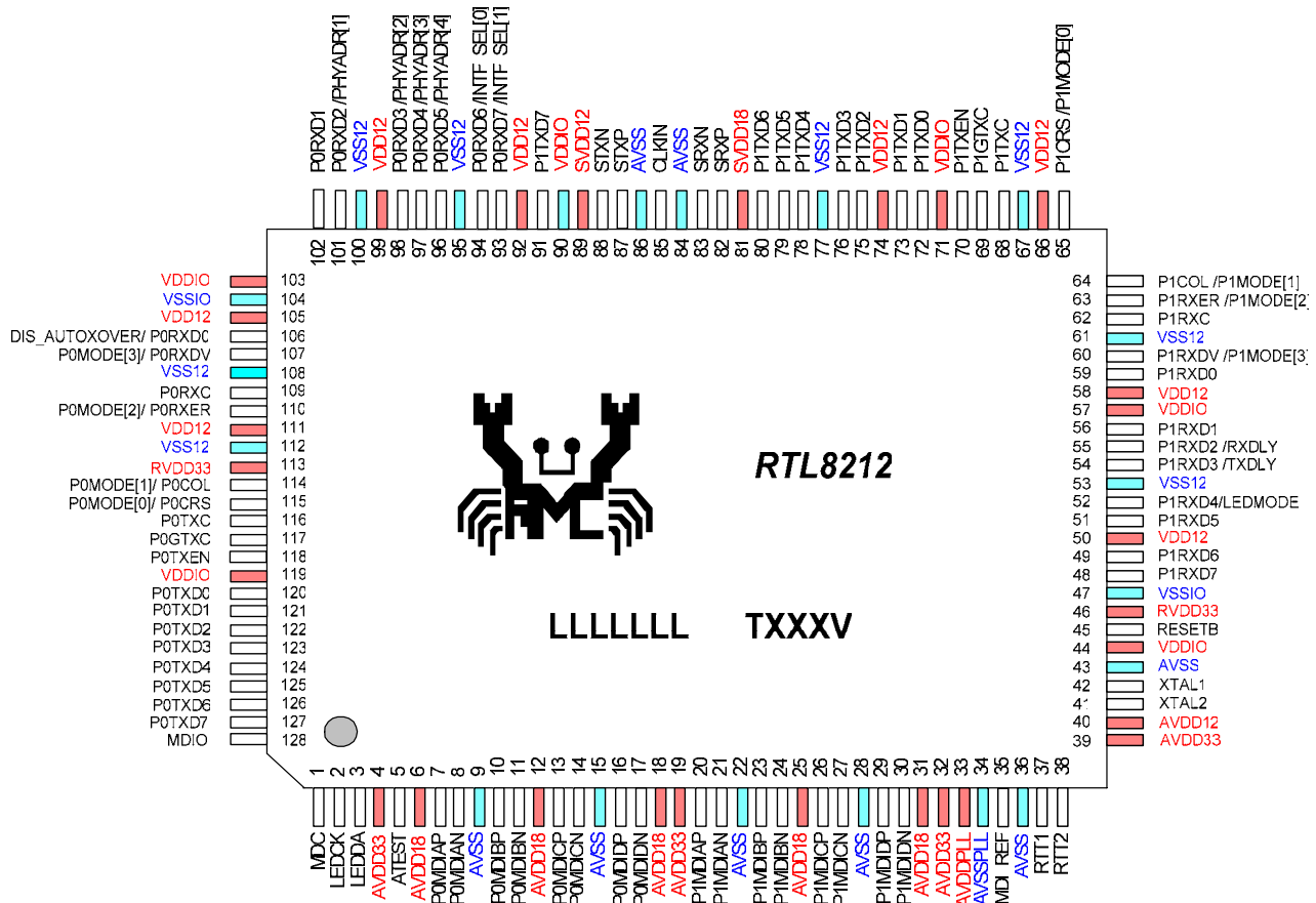
Figure 4. Pin Assignments (QFP-128)
