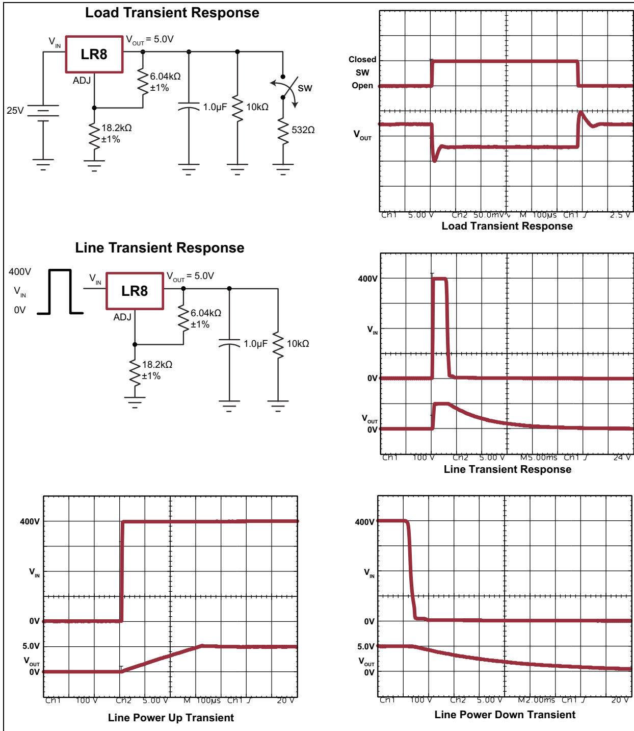
FIGURE 3-7: Typical Performance Curves 3 of 3
