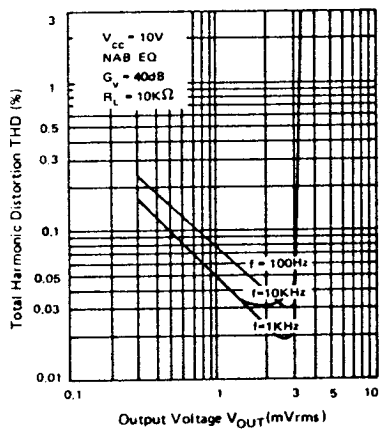
V_{OUT} - THD
