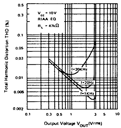
V_{OUT} - THD
