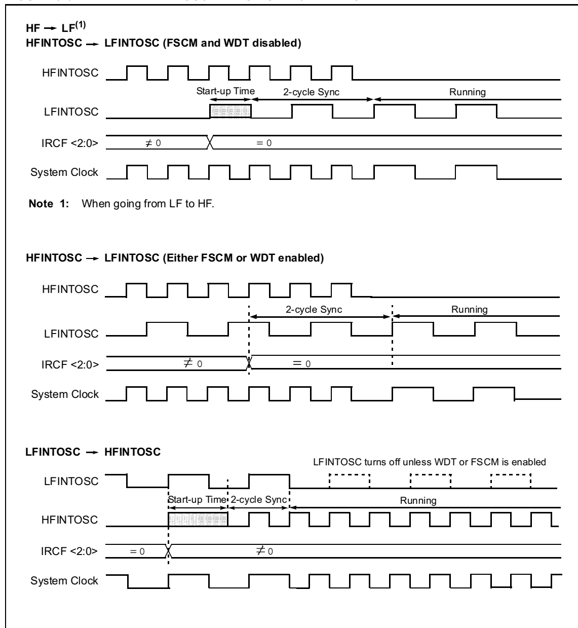
FIGURE 3-6: INTERNAL OSCILLATOR SWITCH TIMING
