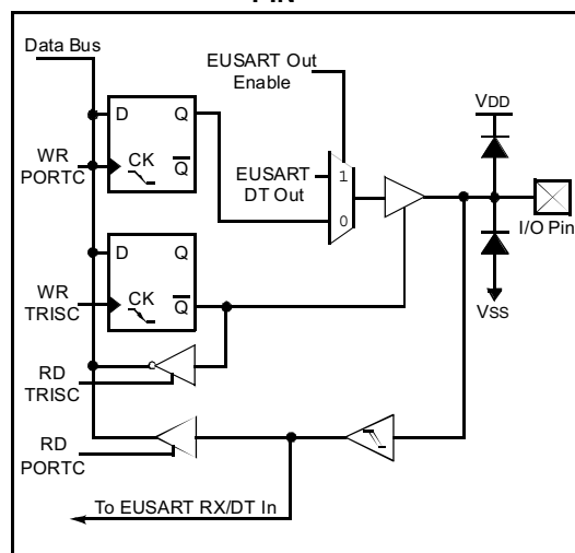
FIGURE 4-10: BLOCK DIAGRAM OF RC5 PIN
