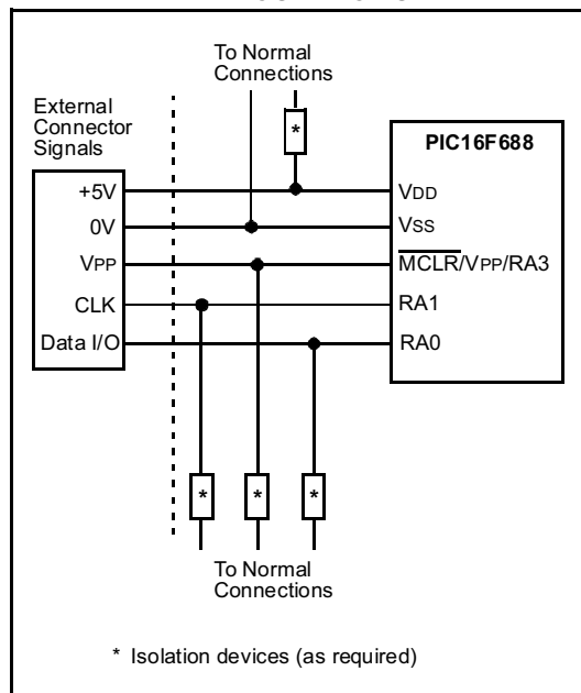
FIGURE 11-11: TYPICAL IN-CIRCUIT SERIAL PROGRAMMING CONNECTION
