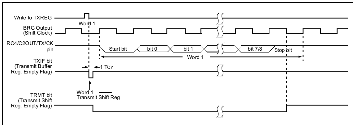
FIGURE 10-3: ASYNCHRONOUS TRANSMISSION
