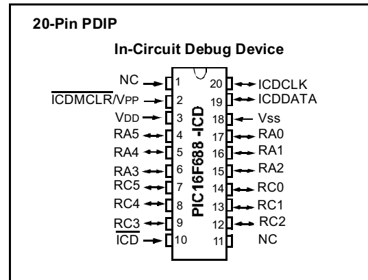
FIGURE 11-12: 20-PIN ICD PINOUT
