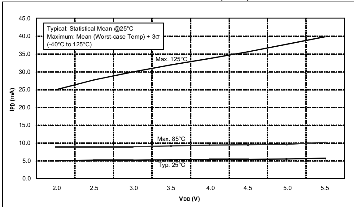
FIGURE 15-29: T1OSC I_{PD} vs. V_{DD} OVER TEMPERATURE (32 kHz)
