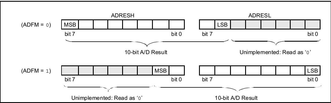
FIGURE 8-3: 10-BIT A/D CONVERSION RESULT FORMAT
