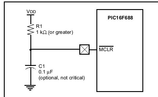
FIGURE 11-2: RECOMMENDED \overline{\text{MCLR}} CIRCUIT
