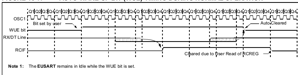
FIGURE 10-7: AUTO-WAKE-UP BIT (WUE) TIMING DURING NORMAL OPERATION
