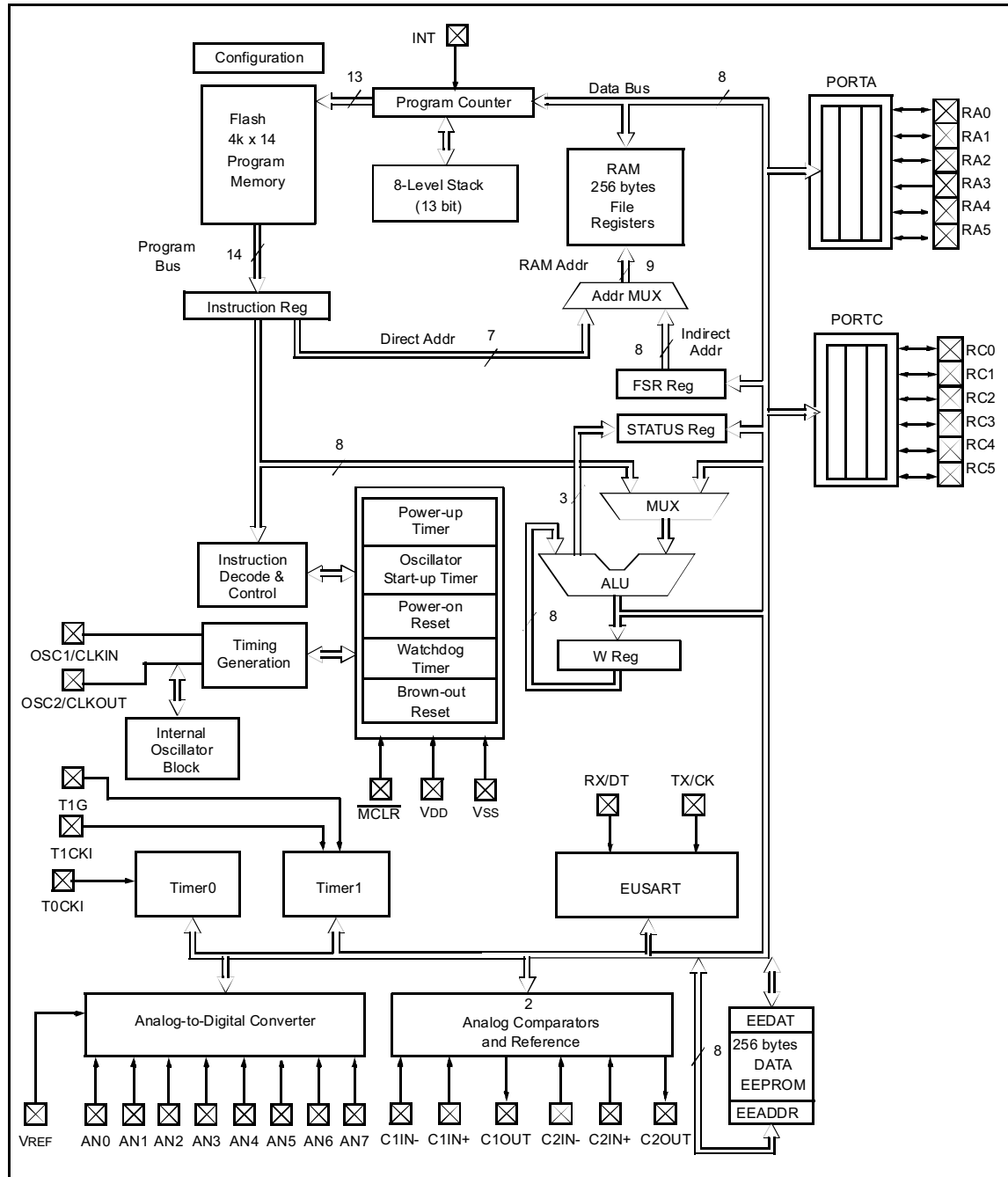
FIGURE 1-1: PIC16F688 BLOCK DIAGRAM
