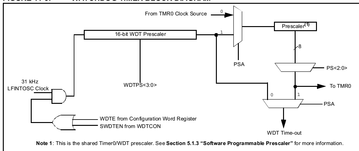
FIGURE 11-9: WATCHDOG TIMER BLOCK DIAGRAM
