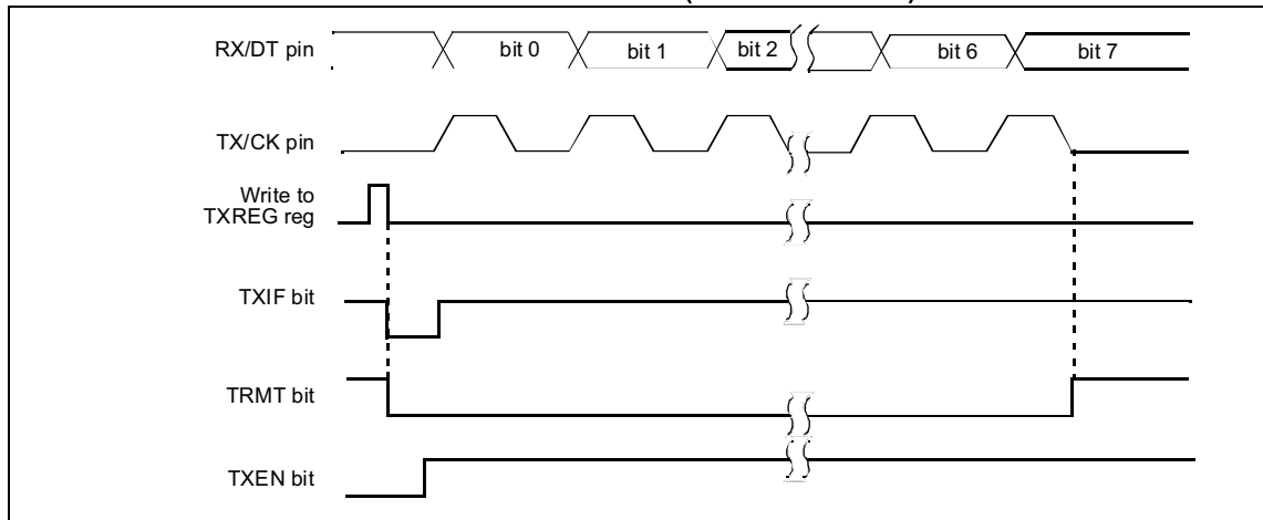
FIGURE 10-11: SYNCHRONOUS TRANSMISSION (THROUGH TXEN)
