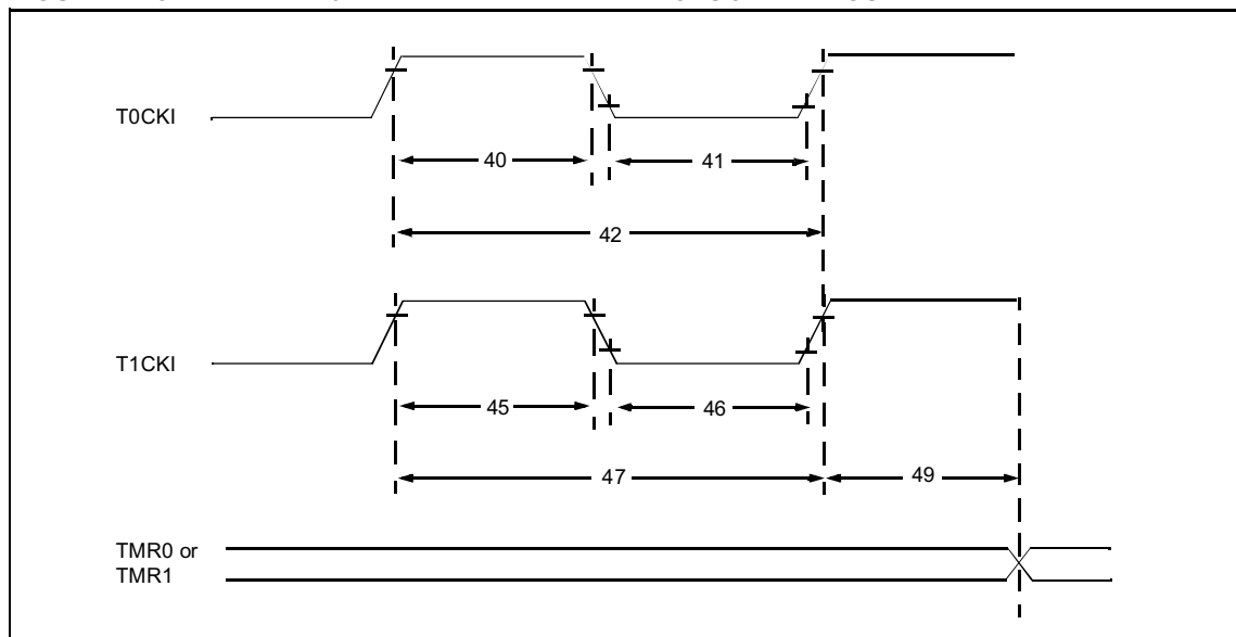
FIGURE 14-8: TIMER0 AND TIMER1 EXTERNAL CLOCK TIMINGS
