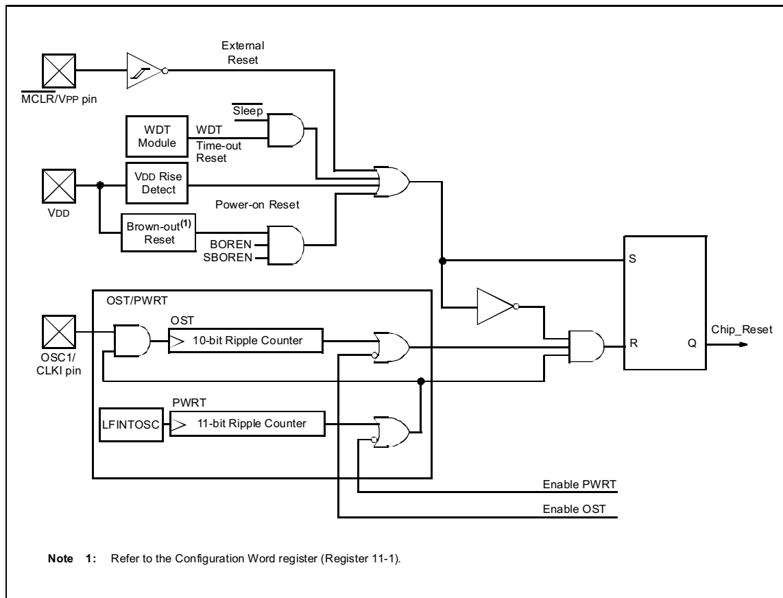
FIGURE 11-1: SIMPLIFIED BLOCK DIAGRAM OF ON-CHIP RESET CIRCUIT
