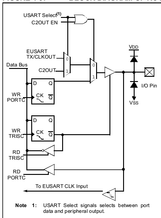
FIGURE 4-9: BLOCK DIAGRAM OF RC4
