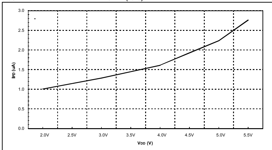
FIGURE 15-17: TYPICAL WDT I_{PD} vs. V_{DD} (25°C)
