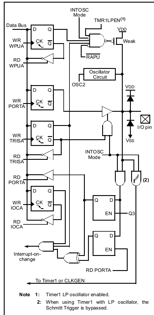
FIGURE 4-6: BLOCK DIAGRAM OF RA5
