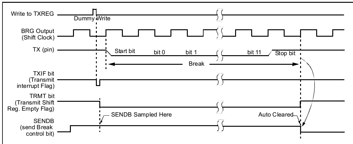
FIGURE 10-9: SEND BREAK CHARACTER SEQUENCE
