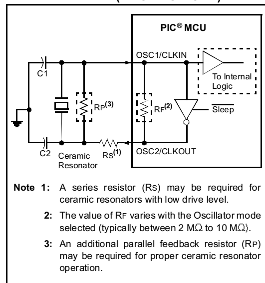
FIGURE 3-4: CERAMIC RESONATOR OPERATION (XT OR HS MODE)
