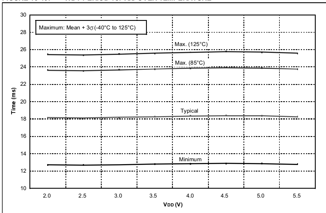
FIGURE 15-19: WDT PERIOD vs. VDD OVER TEMPERATURE
