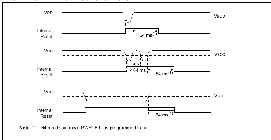
FIGURE 11-3: BROWN-OUT SITUATIONS
