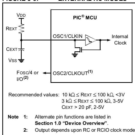
FIGURE 3-5: EXTERNAL RC MODES
