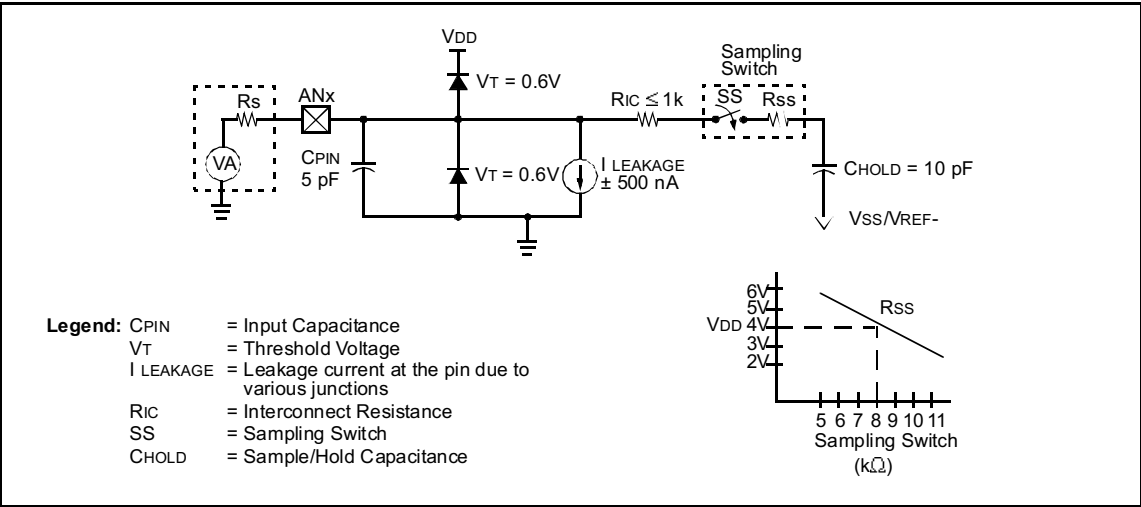
FIGURE 8-4: ANALOG INPUT MODEL
