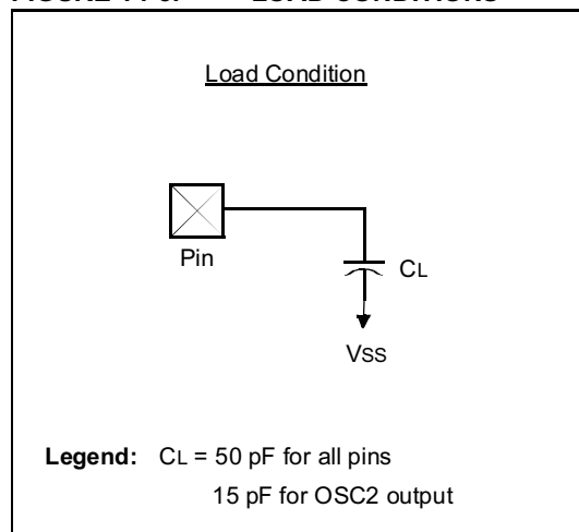
FIGURE 14-3: LOAD CONDITIONS
