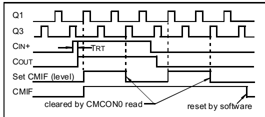
FIGURE 7-7: COMPARATOR INTERRUPT TIMING WITH CMCON0 READ
