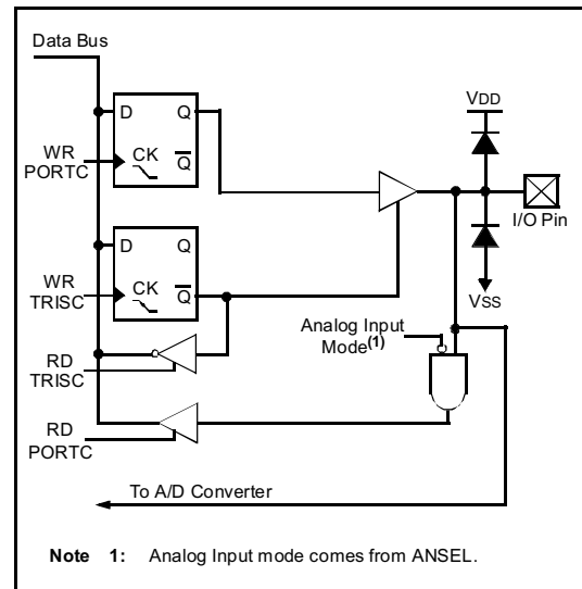
FIGURE 4-8: BLOCK DIAGRAM OF RC2 AND RC3
