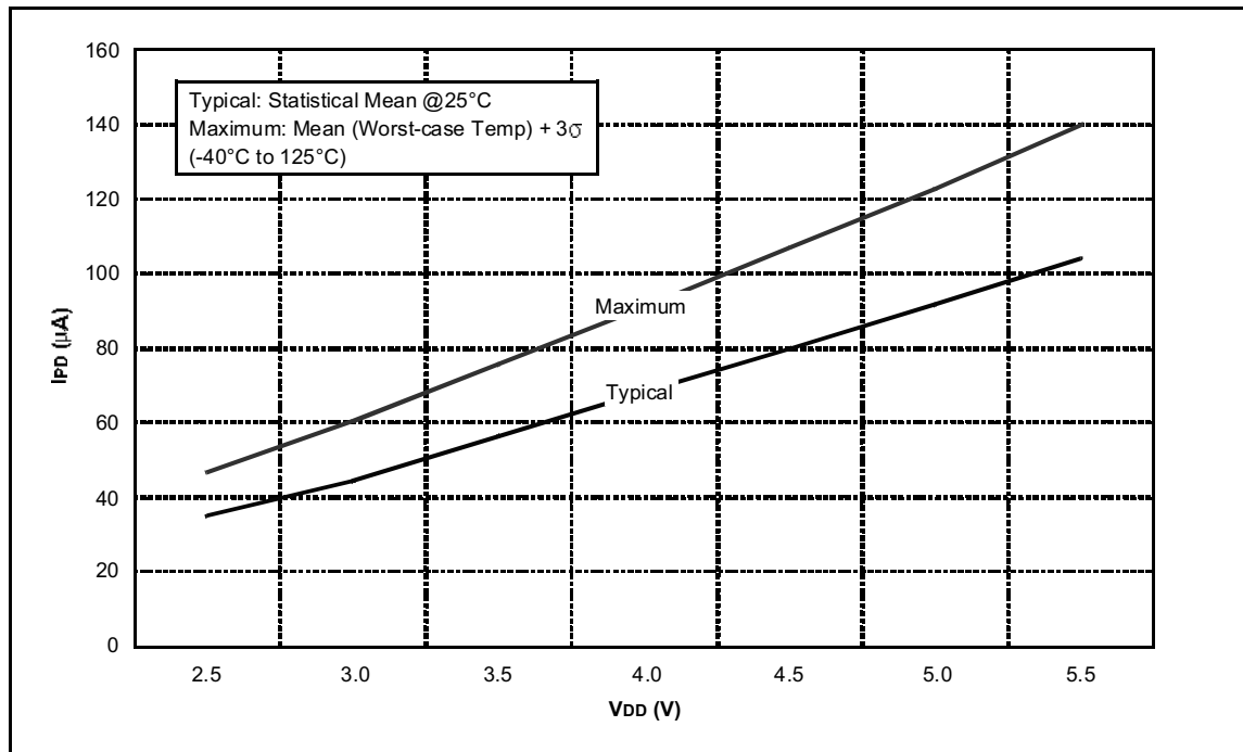
FIGURE 15-16: BOR I_{PD} vs. V_{DD} OVER TEMPERATURE
