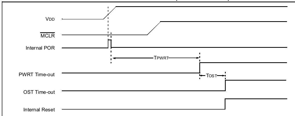
FIGURE 11-5: TIME-OUT SEQUENCE ON POWER-UP (DELAYED \overline{\text{MCLR}} )
