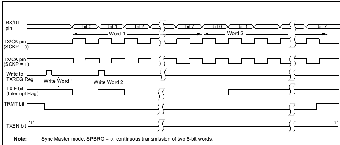
FIGURE 10-10: SYNCHRONOUS TRANSMISSION
