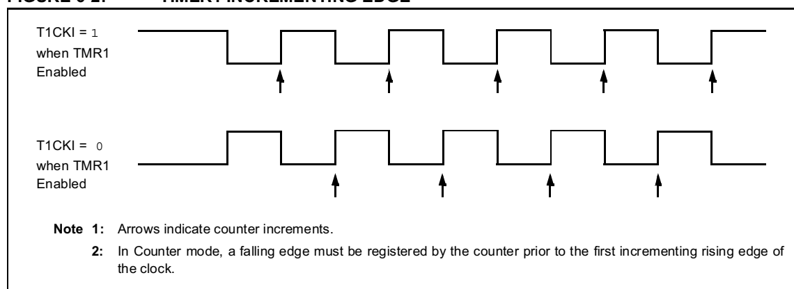
FIGURE 6-2: TIMER1 INCREMENTING EDGE
