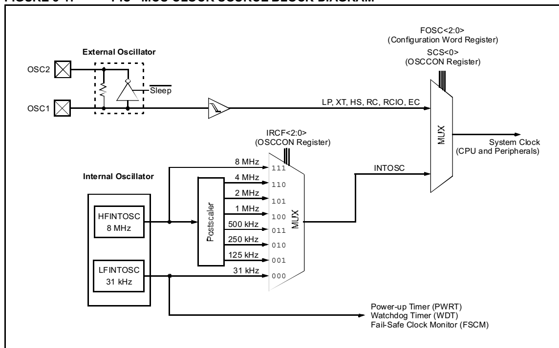
FIGURE 3-1: PIC® MCU CLOCK SOURCE BLOCK DIAGRAM
