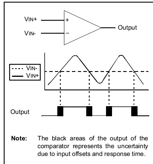
FIGURE 7-1: SINGLE COMPARATOR
