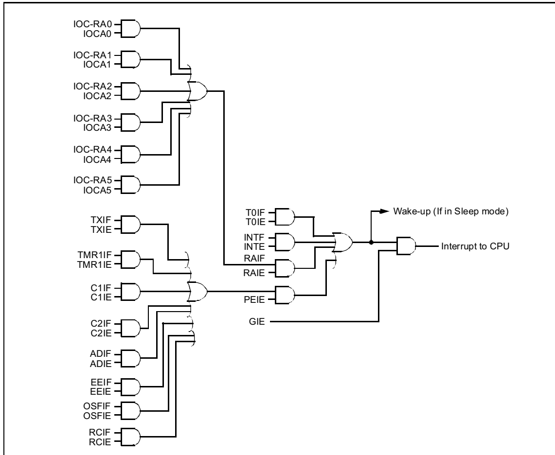
FIGURE 11-7: INTERRUPT LOGIC
