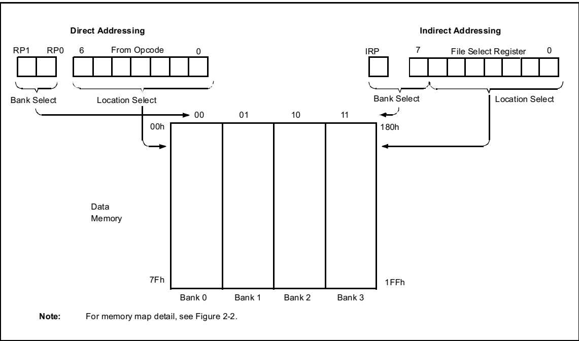
FIGURE 2-4: DIRECT/INDIRECT ADDRESSING PIC16F688
