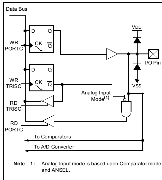
FIGURE 4-7: BLOCK DIAGRAM OF RC0 AND RC1
