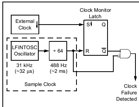
FIGURE 3-8: FSCM BLOCK DIAGRAM
