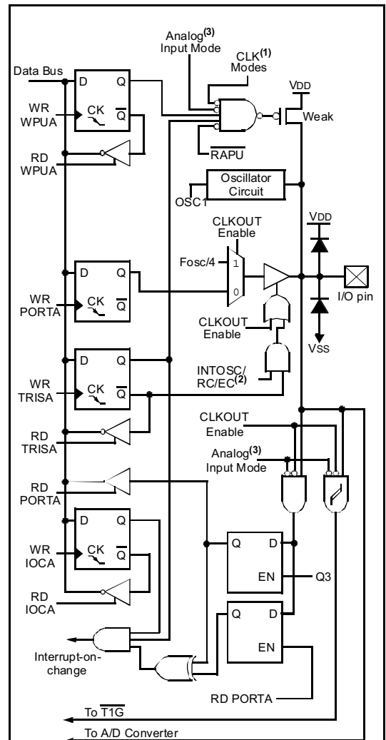
FIGURE 4-5: BLOCK DIAGRAM OF RA4
