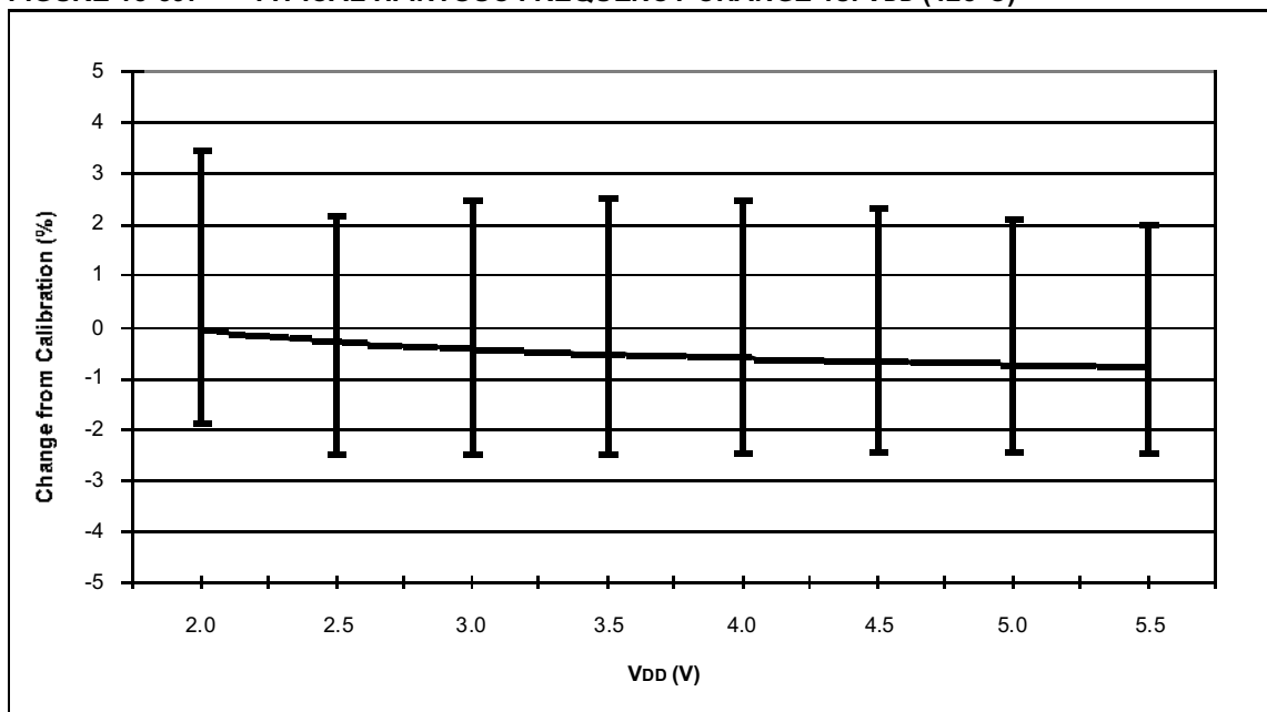
FIGURE 15-39: TYPICAL HFINTOSC FREQUENCY CHANGE vs. V_{DD} (125°C)
