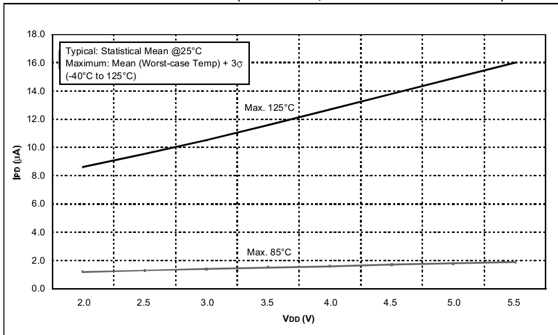
FIGURE 15-15: COMPARATOR I_{PD} vs. V_{DD} (BOTH COMPARATORS ENABLED)
