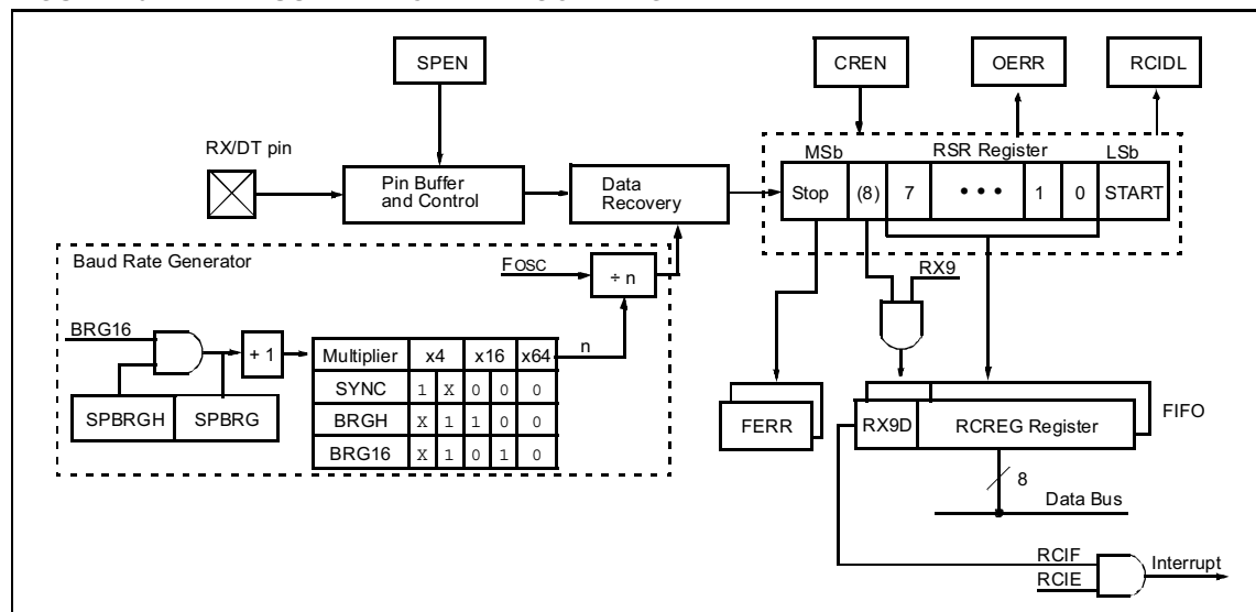
FIGURE 10-2: EUSART RECEIVE BLOCK DIAGRAM
