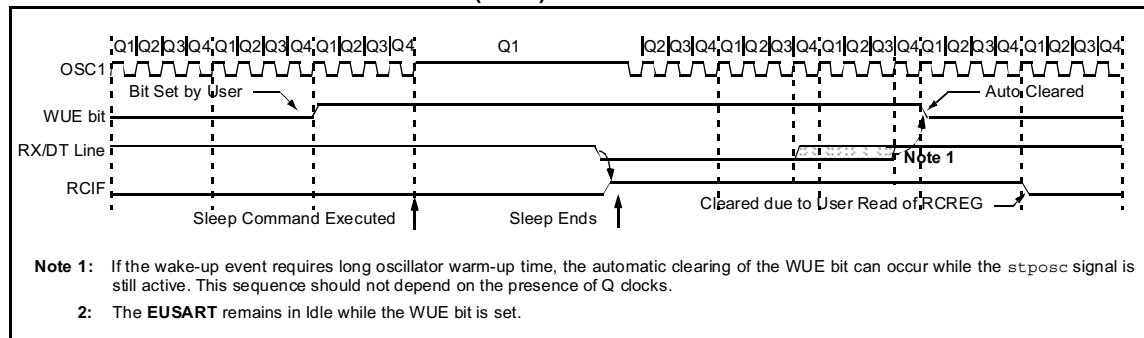
FIGURE 10-8: AUTO-WAKE-UP BIT (WUE) TIMINGS DURING SLEEP
