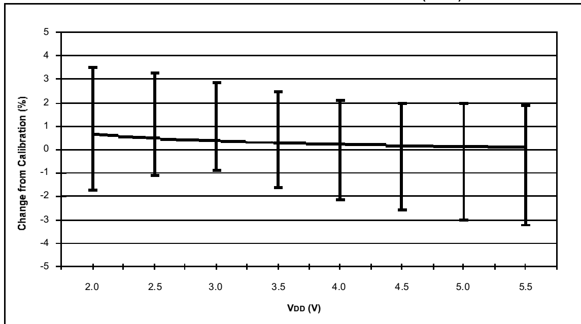
FIGURE 15-40: TYPICAL HFINTOSC FREQUENCY CHANGE vs. V_{DD} ( -40^{\circ}\text{C} )
