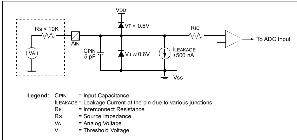
FIGURE 7-4: ANALOG INPUT MODEL
