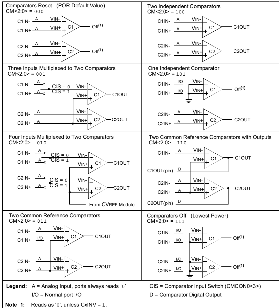
FIGURE 7-5: COMPARATOR I/O OPERATING MODES
