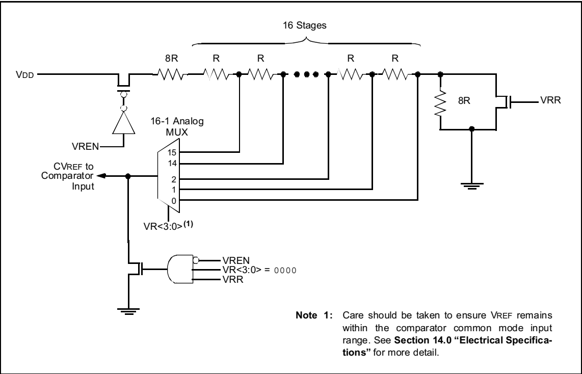
FIGURE 7-8: COMPARATOR VOLTAGE REFERENCE BLOCK DIAGRAM
