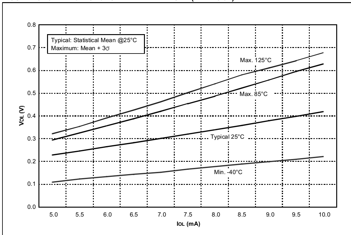
FIGURE 15-23: VOL vs. IOL OVER TEMPERATURE (VDD = 3.0V)
