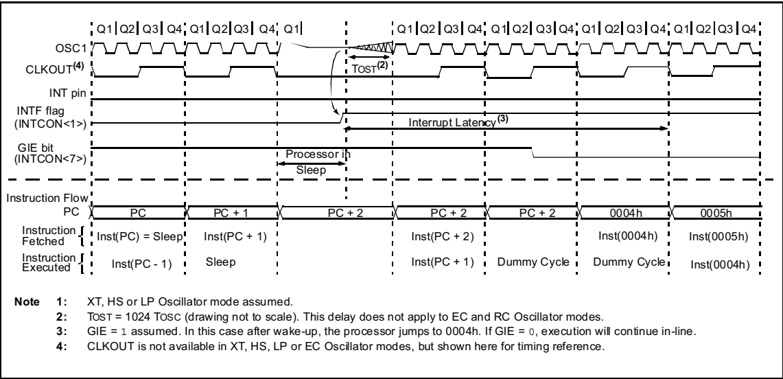
FIGURE 11-10: WAKE-UP FROM SLEEP THROUGH INTERRUPT
