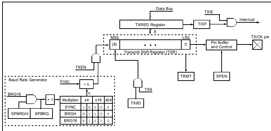
FIGURE 10-1: EUSART TRANSMIT BLOCK DIAGRAM
