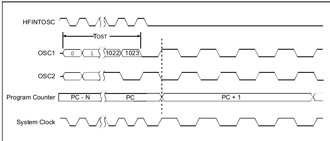
FIGURE 3-7: TWO-SPEED START-UP
