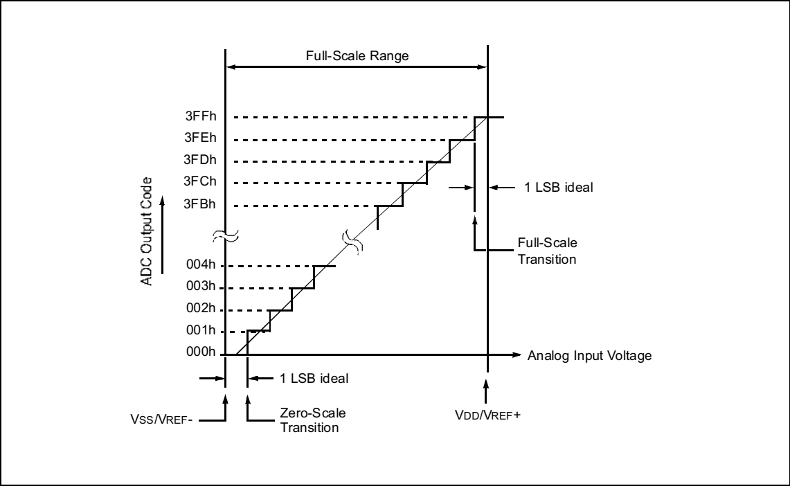
FIGURE 8-5: ADC TRANSFER FUNCTION
