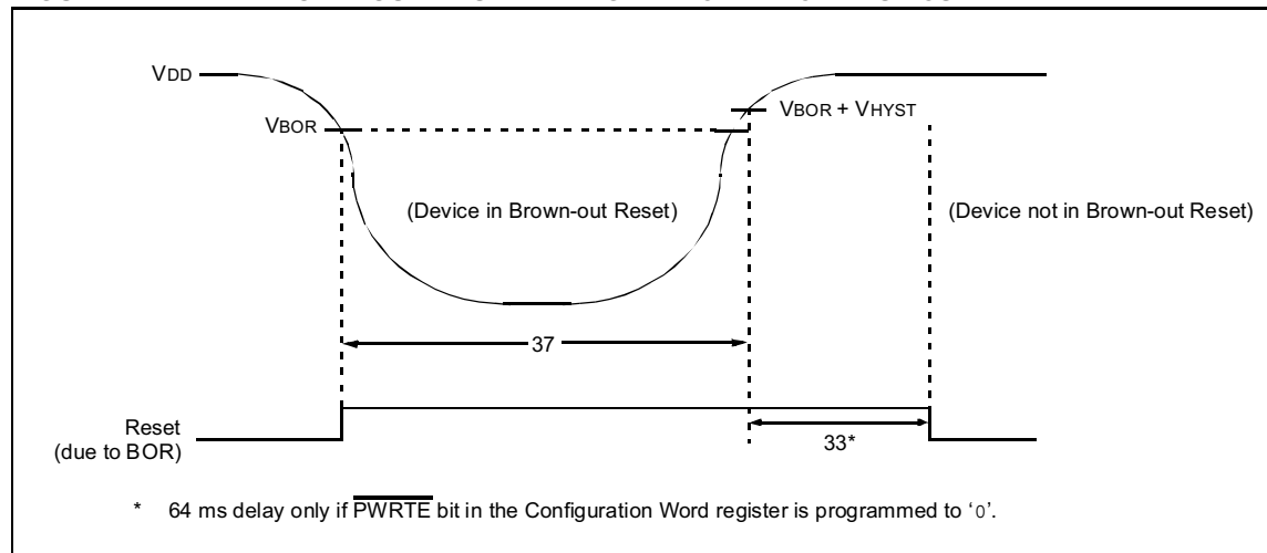
FIGURE 14-7: BROWN-OUT RESET TIMING AND CHARACTERISTICS
