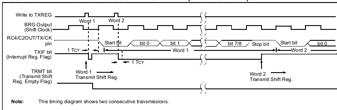
FIGURE 10-4: ASYNCHRONOUS TRANSMISSION (BACK-TO-BACK)
