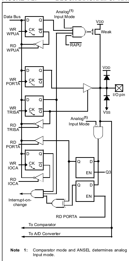
FIGURE 4-2: BLOCK DIAGRAM OF RA1
