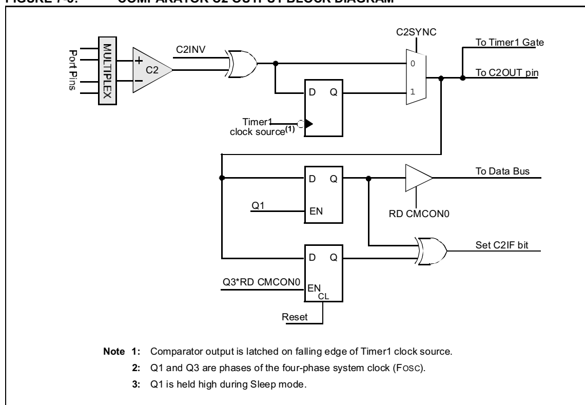
FIGURE 7-3: COMPARATOR C2 OUTPUT BLOCK DIAGRAM
