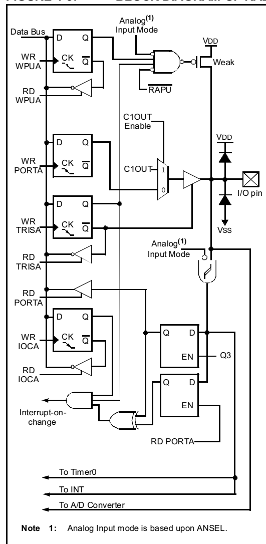
FIGURE 4-3: BLOCK DIAGRAM OF RA2
