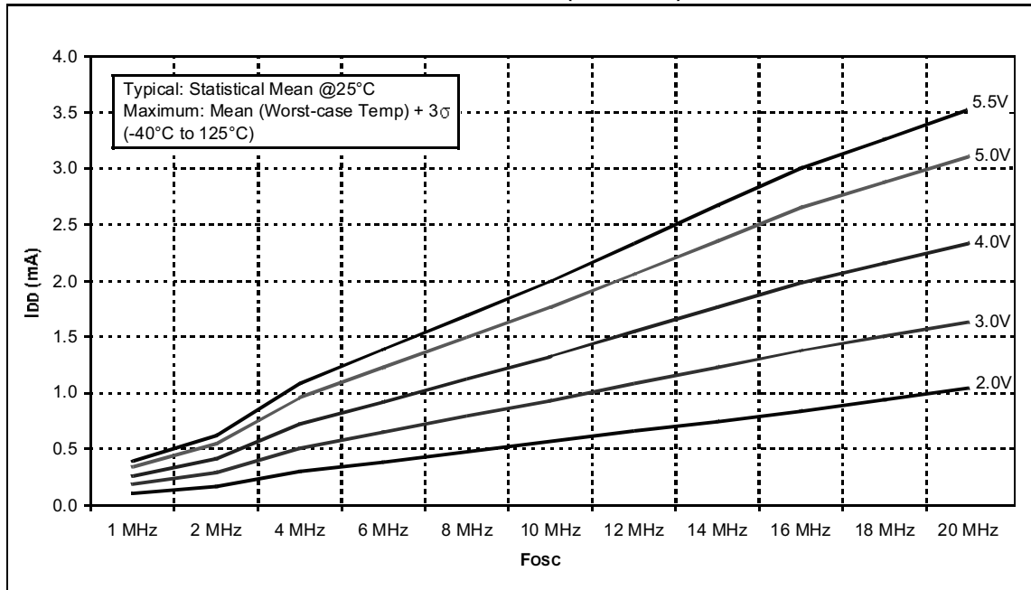
FIGURE 15-3: TYPICAL I_{DD} vs. F_{osc} OVER V_{DD} (HS MODE)
