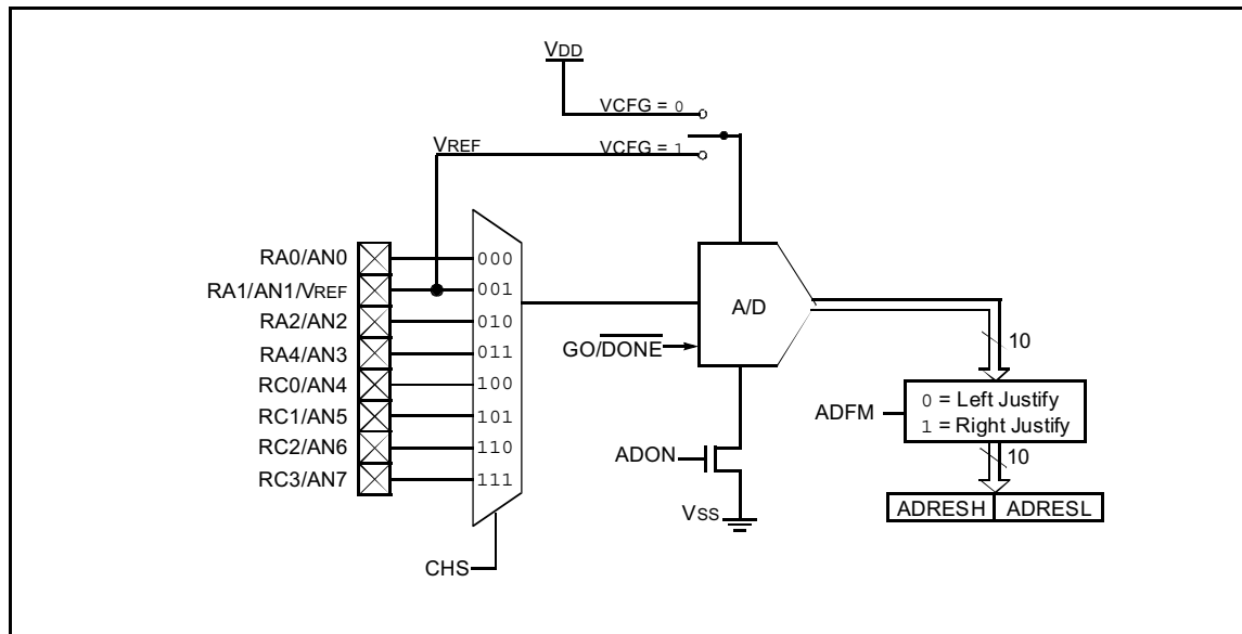
FIGURE 8-1: ADC BLOCK DIAGRAM
