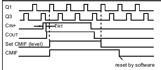
FIGURE 7-7: COMPARATOR INTERRUPT TIMING WITH CMCON0 READ
