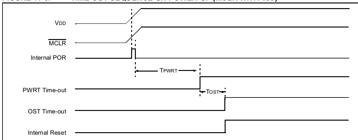
FIGURE 11-6: TIME-OUT SEQUENCE ON POWER-UP ( \overline{\text{MCLR}} WITH V_{DD} )
