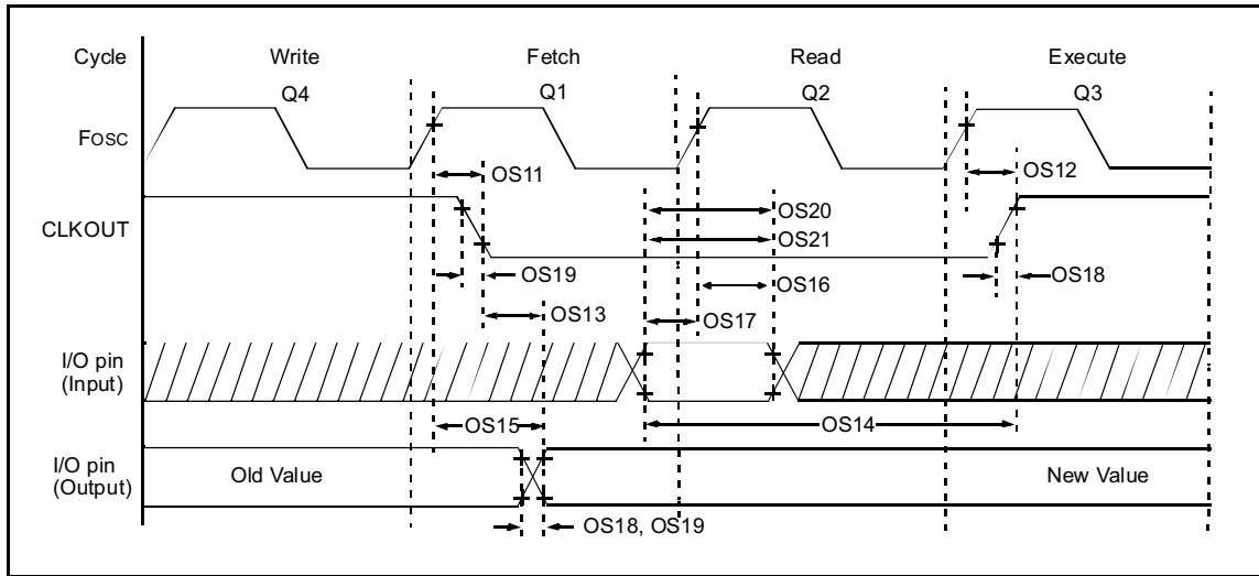
FIGURE 14-5: CLKOUT AND I/O TIMING
