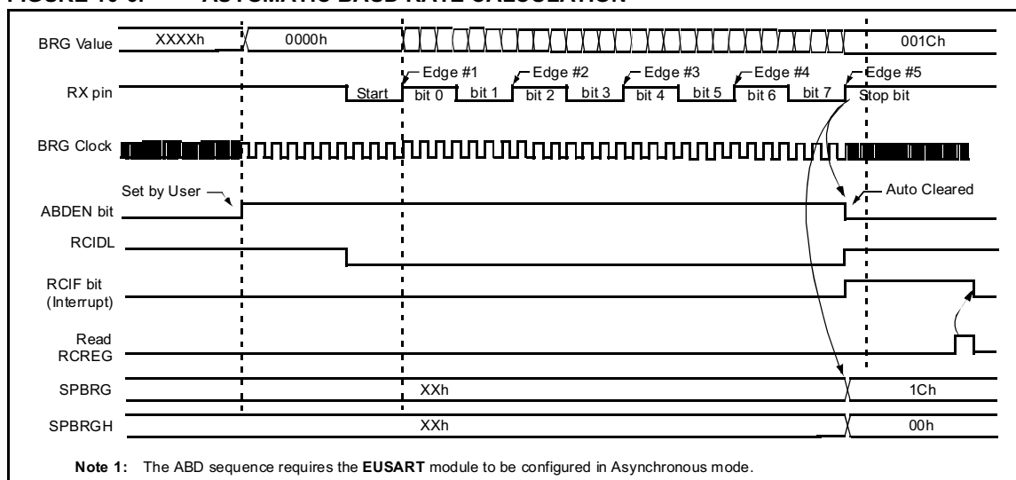
FIGURE 10-6: AUTOMATIC BAUD RATE CALCULATION
