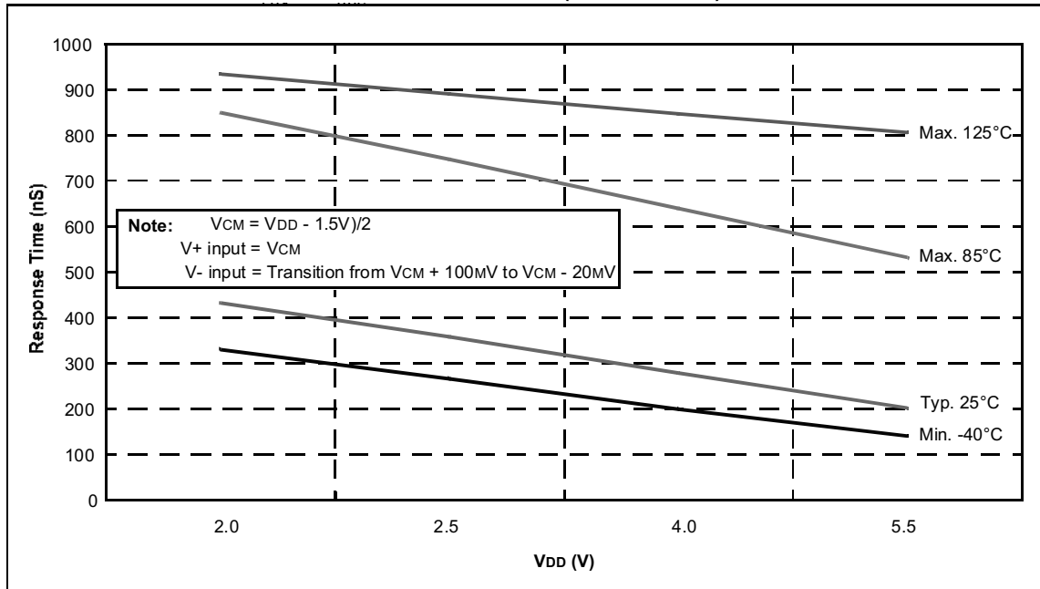
FIGURE 15-30: COMPARATOR RESPONSE TIME (RISING EDGE)
