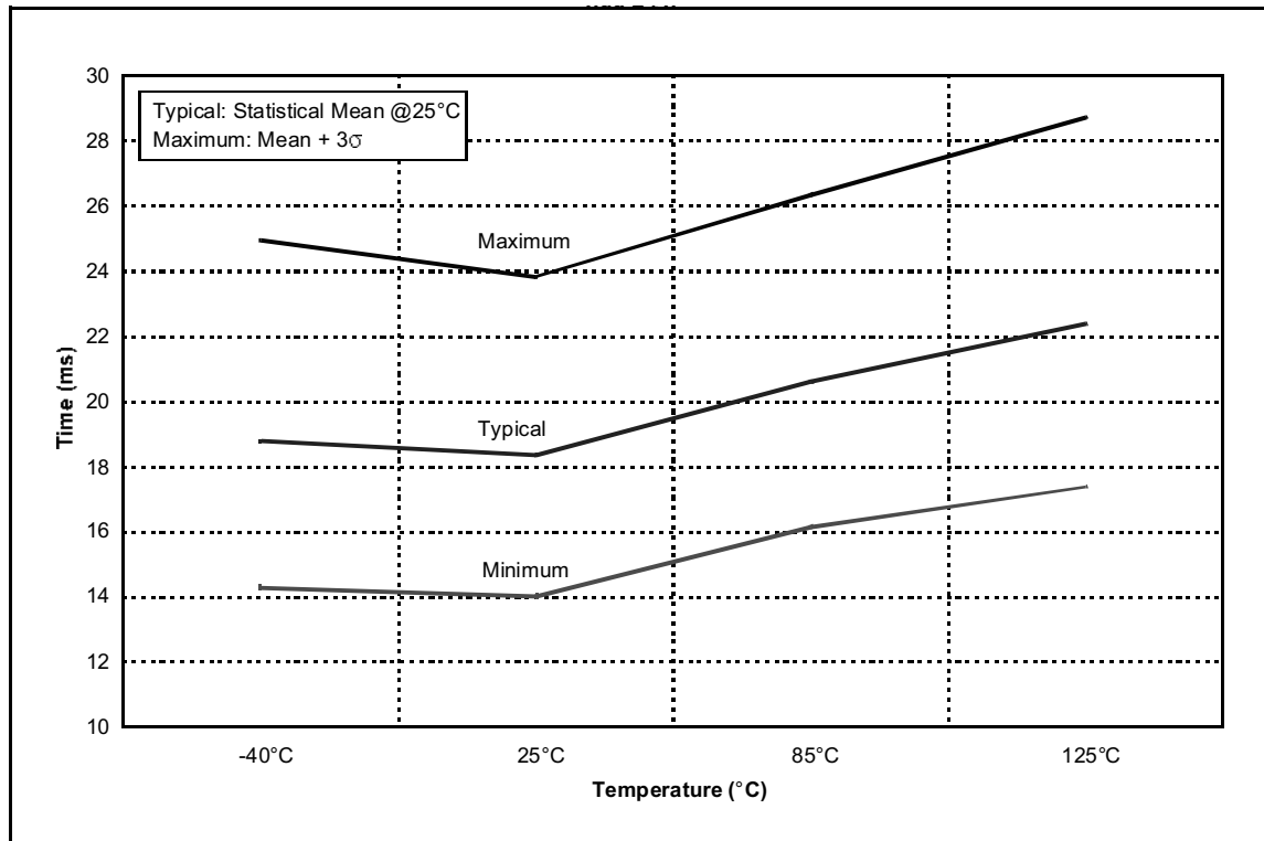
FIGURE 15-20: WDT PERIOD vs. TEMPERATURE
