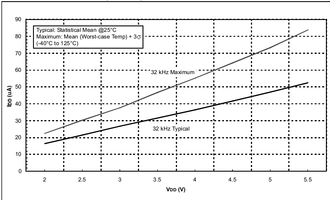
FIGURE 15-10: I_{DD} vs. V_{DD} (LP MODE)
