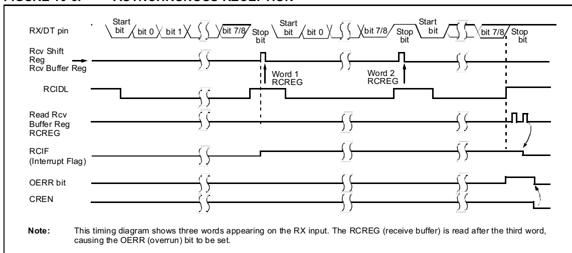
FIGURE 10-5: ASYNCHRONOUS RECEPTION
