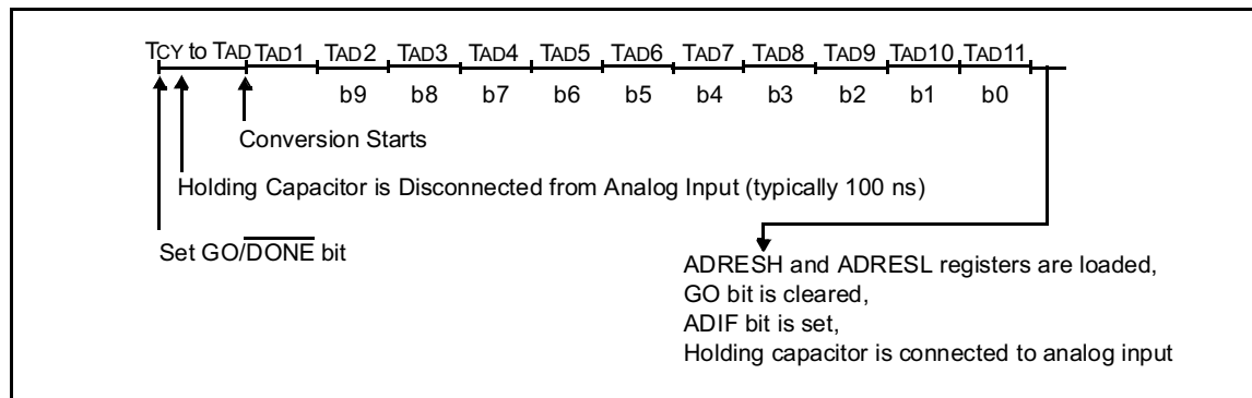
FIGURE 8-2: ANALOG-TO-DIGITAL CONVERSION T AD CYCLES
