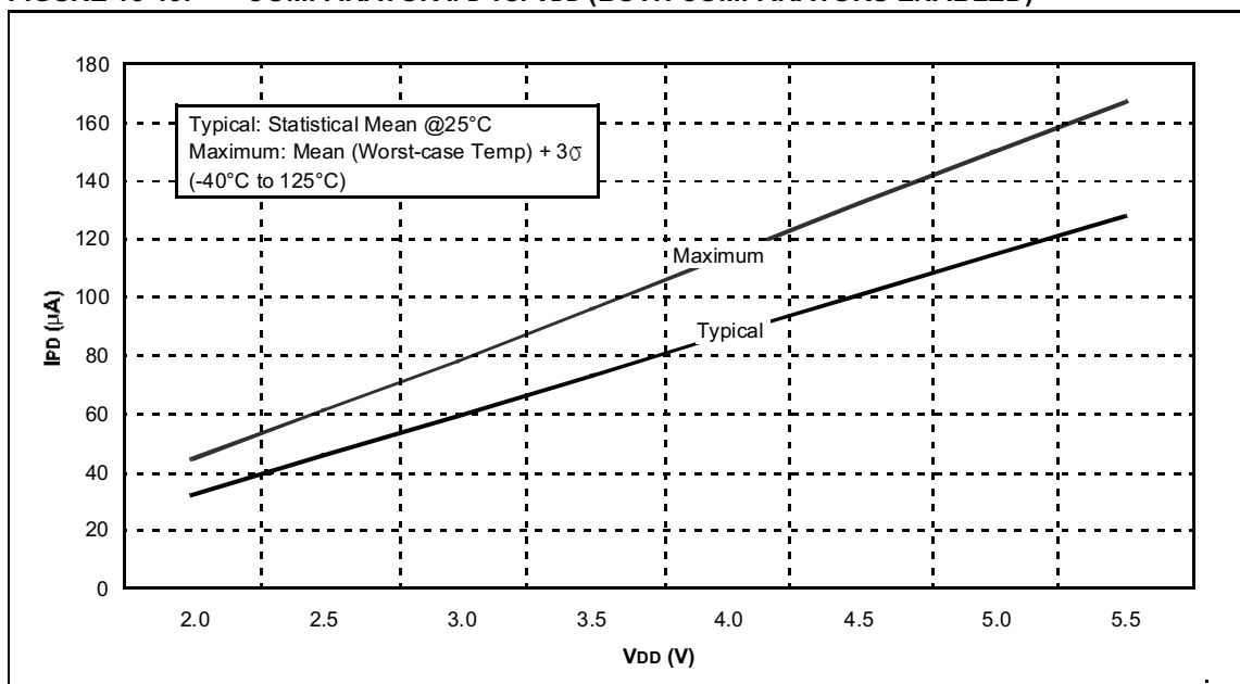
FIGURE 15-15: COMPARATOR I_{PD} vs. V_{DD} (BOTH COMPARATORS ENABLED)
