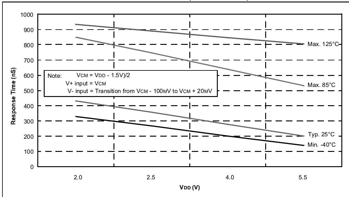
FIGURE 15-31: COMPARATOR RESPONSE TIME (FALLING EDGE)
